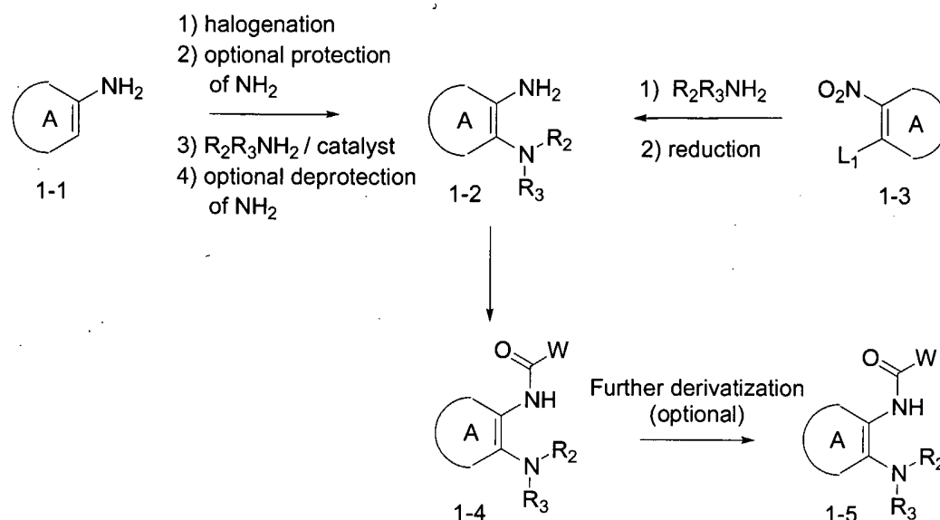
Scheme 1 illustrates general methodology for the preparation of compounds of Formula I.
