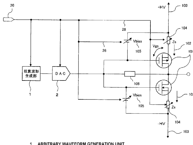
1 ARBITRARY WAVEFORM GENERATION UNIT
