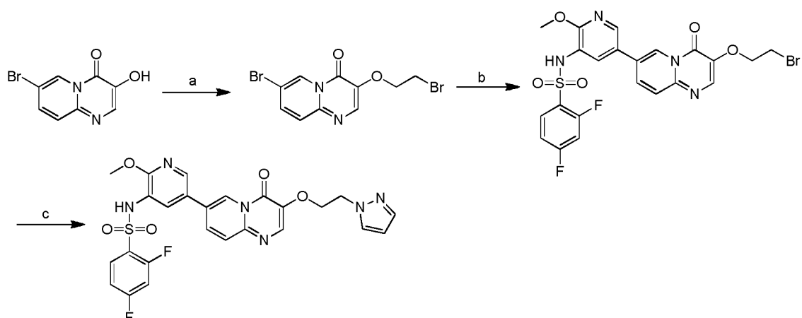
Scheme 4:
