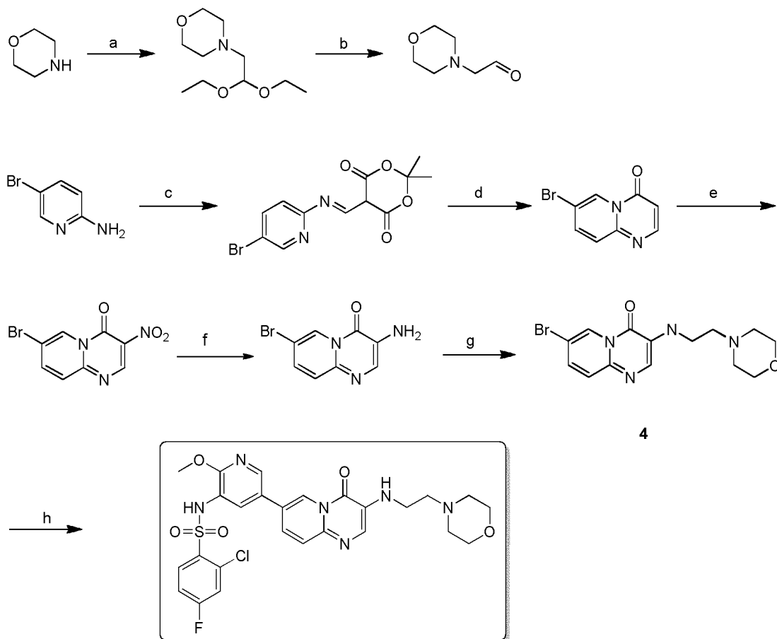
Scheme 14:
