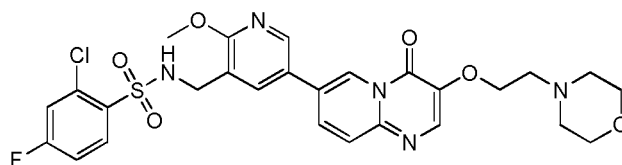
Compound 99
