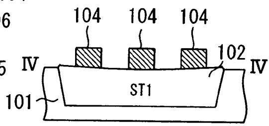
Fig. 13C (PRIOR ART)
