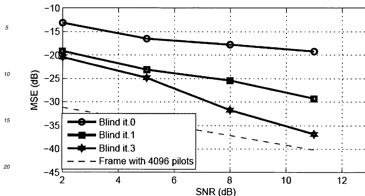
Fig. 5. MSE in dB of the channel estimation error.
