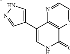
Compound 576
