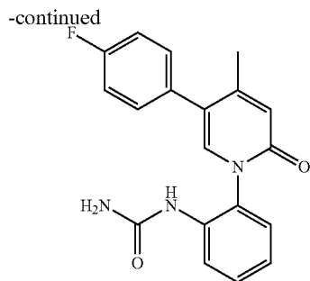
Compound 557
