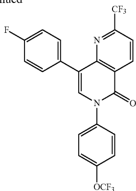
Compound 38
