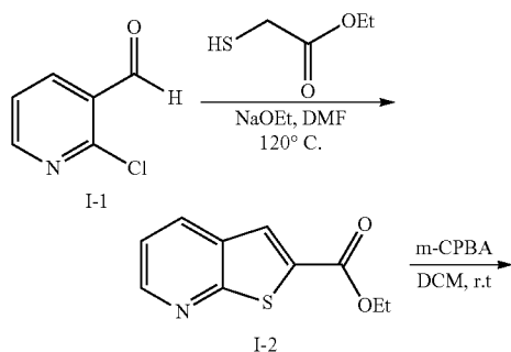
Synthesis of Compound 1 (Scheme I)
