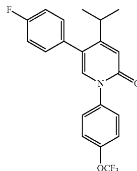
Compound 200
