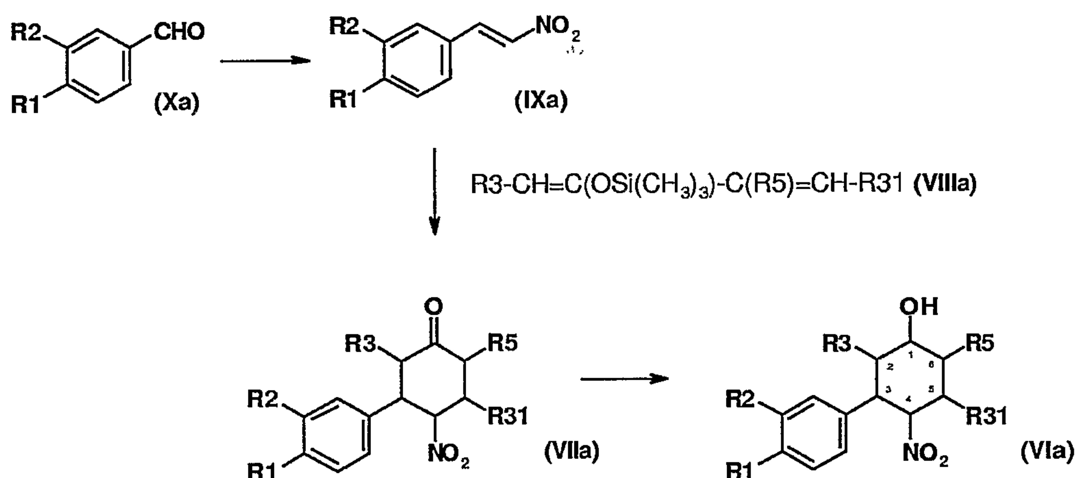
Reaction scheme 2:
