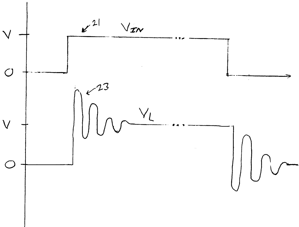
Fig. 2 (Prior Art)
