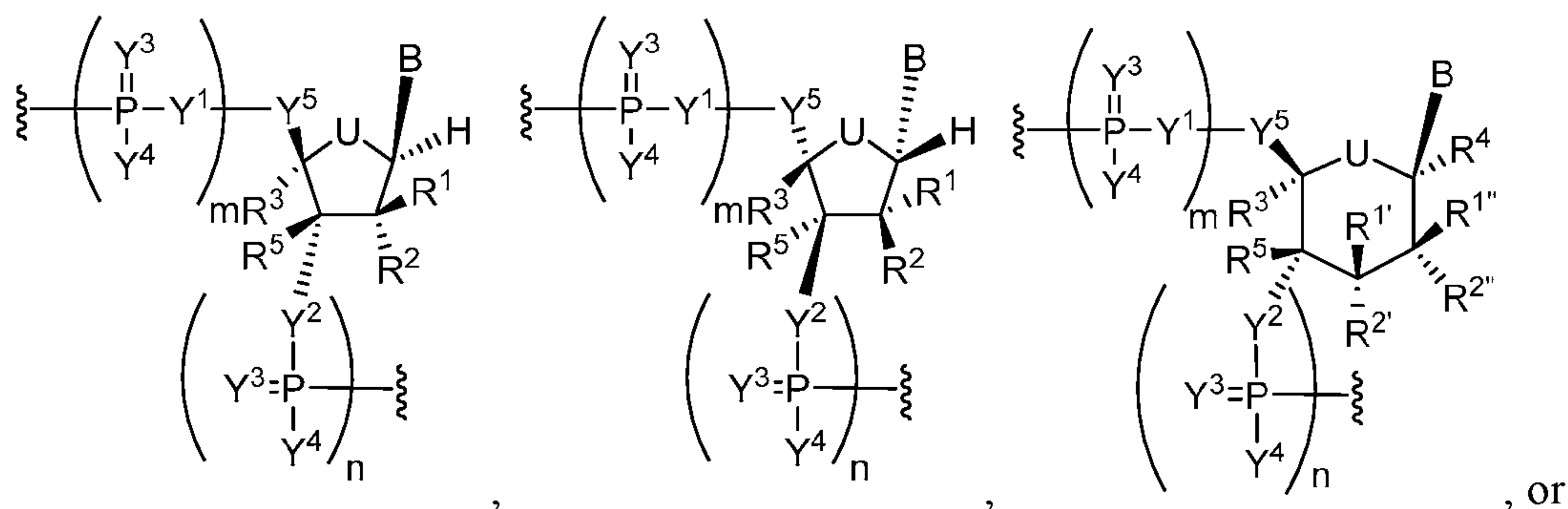
Formula IV
