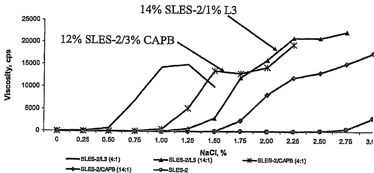
Figure 9 Viscosity v. NaCl% Results
