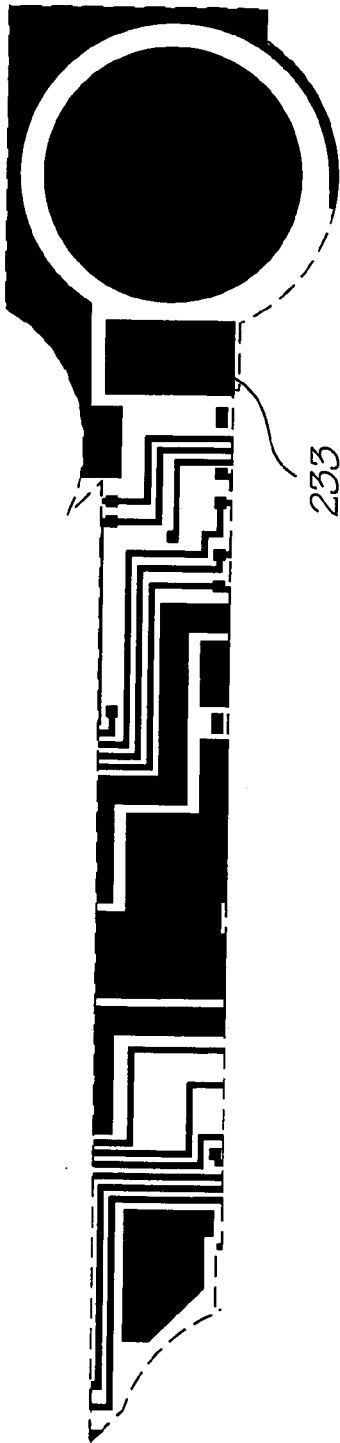
Metal 2 mask
