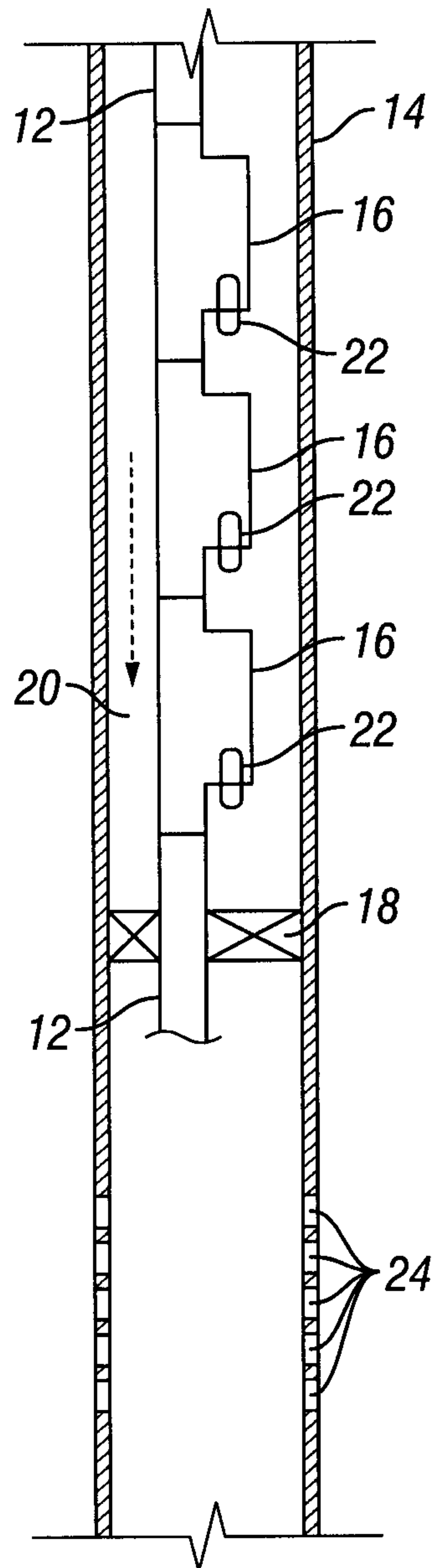
FIG. 1 (Prior Art)
