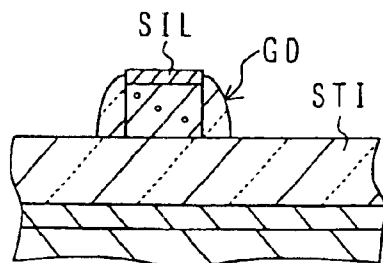
FIG.7C RELATED ART
