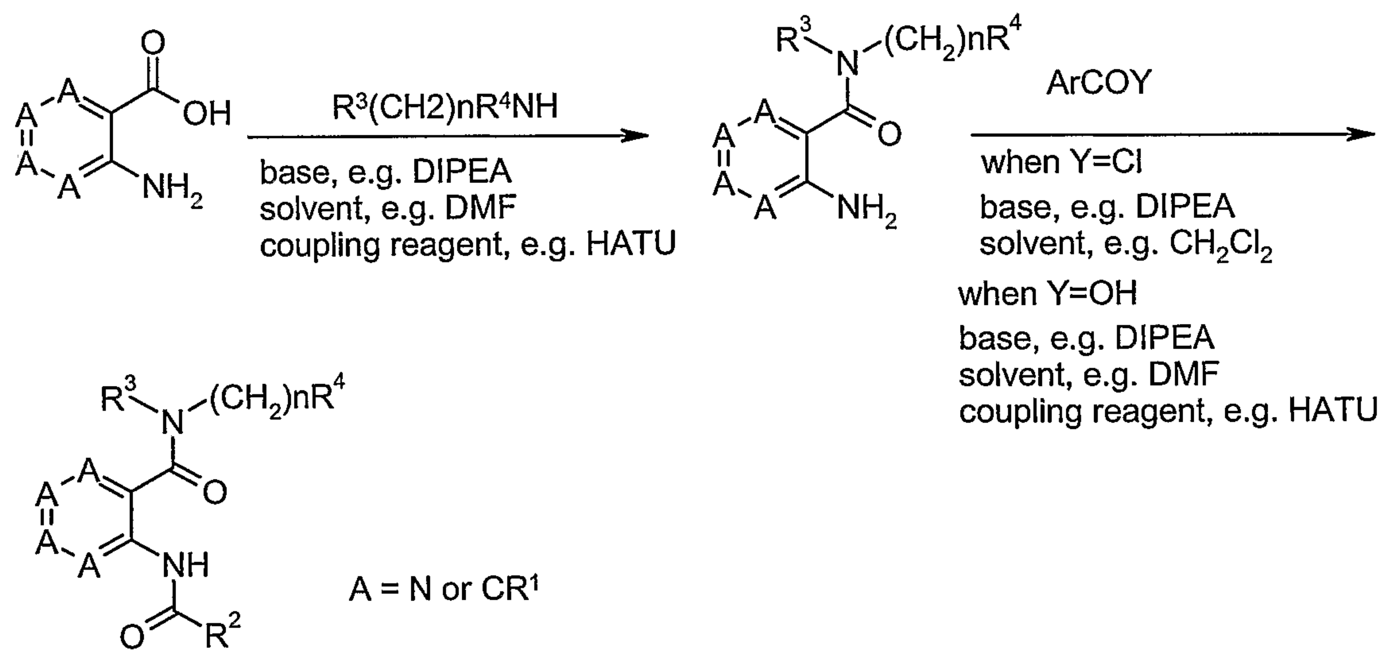
Scheme 2. A synthetic route used for the synthesis of examples
