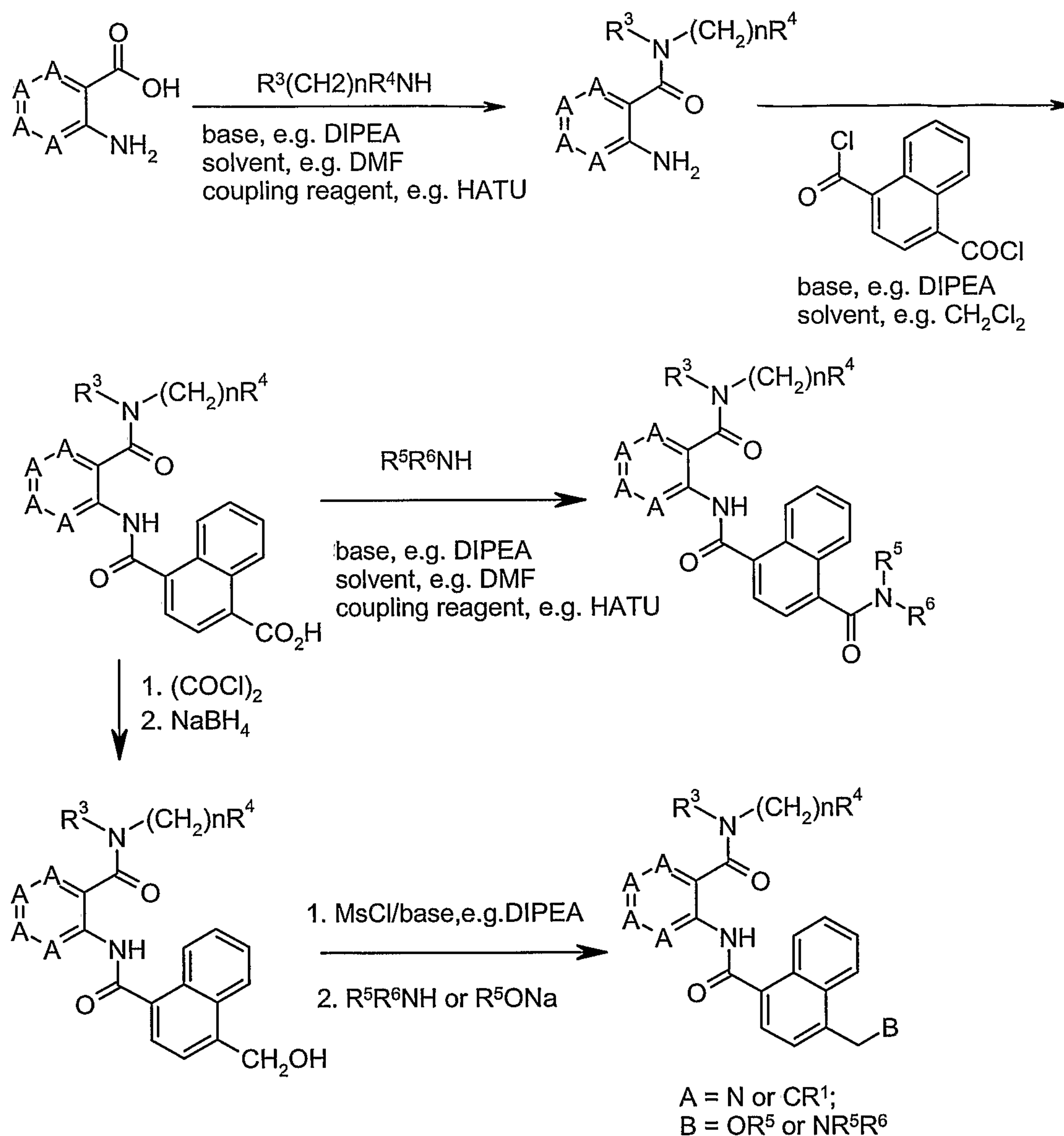
Scheme 5. A synthetic route used for the synthesis of examples
