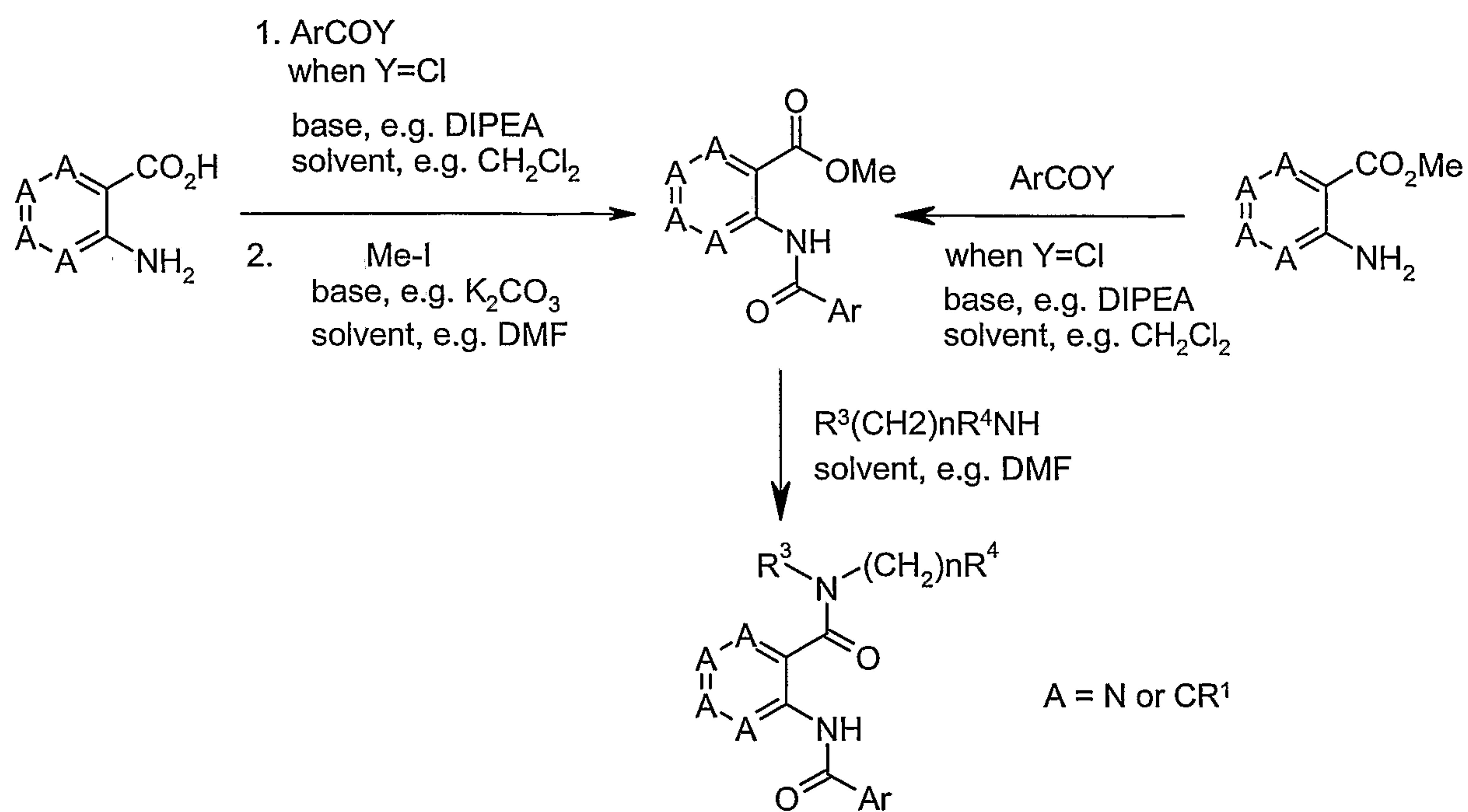
Scheme 3. A synthetic route used for the synthesis of examples
