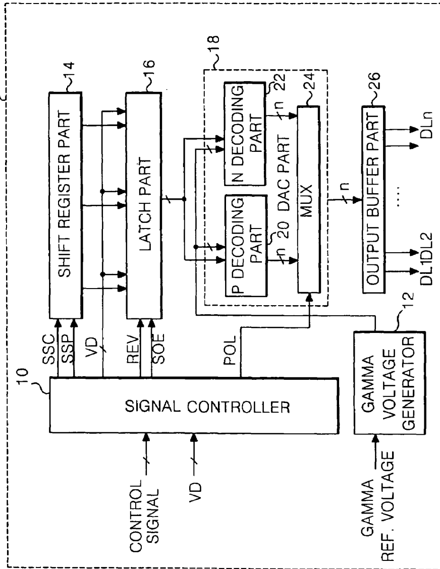
FIG. 2 CONVENTIONAL ART
