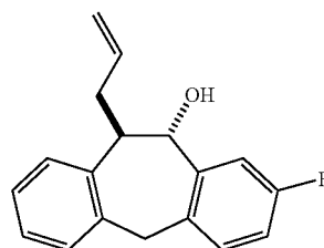
intermediate 55
