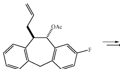
intermediate 56
