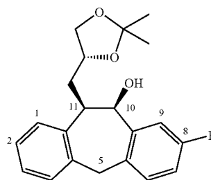
intermediate 3
