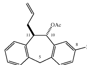
intermediate 56
