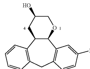
final compound 29
