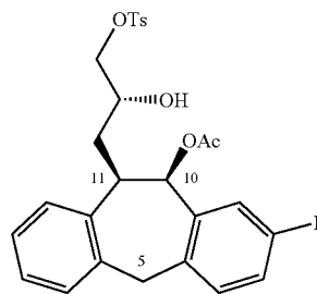
intermediate 23a
