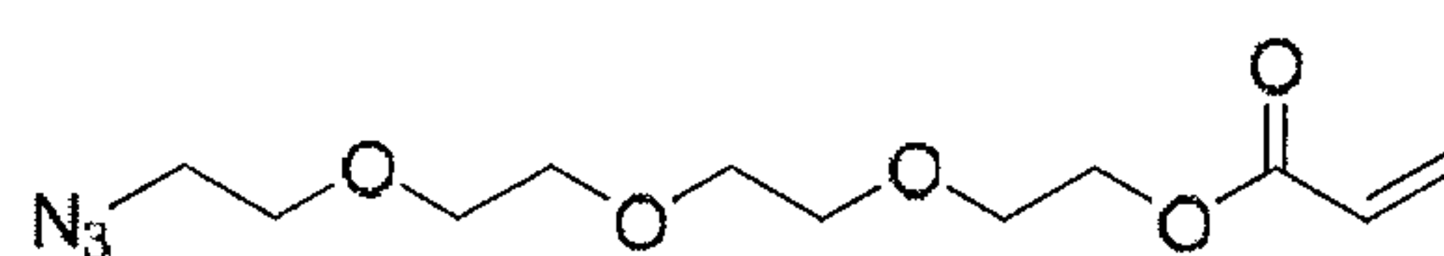
Azide-PEG4-Acrylate
