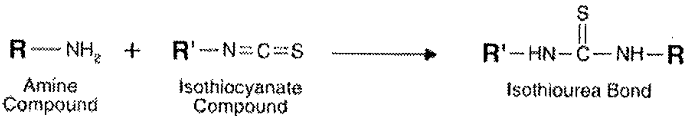
(REACTION 3.1)
