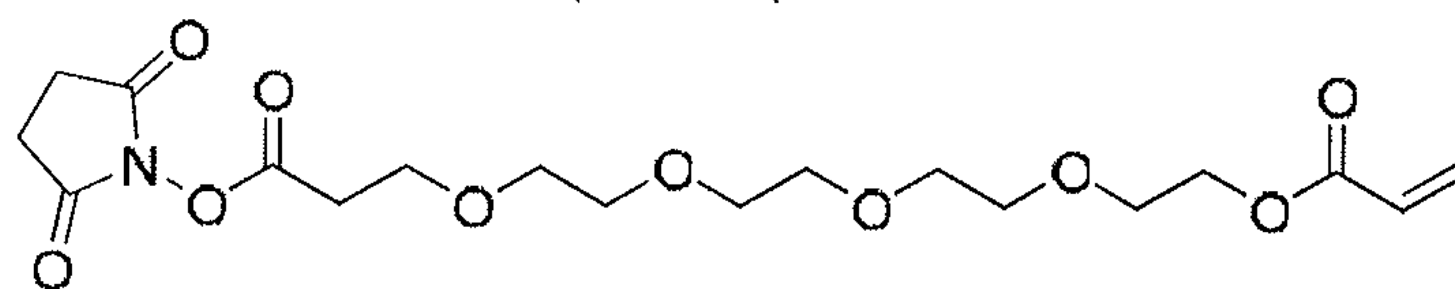
NHS-PEG5-Acrylate
