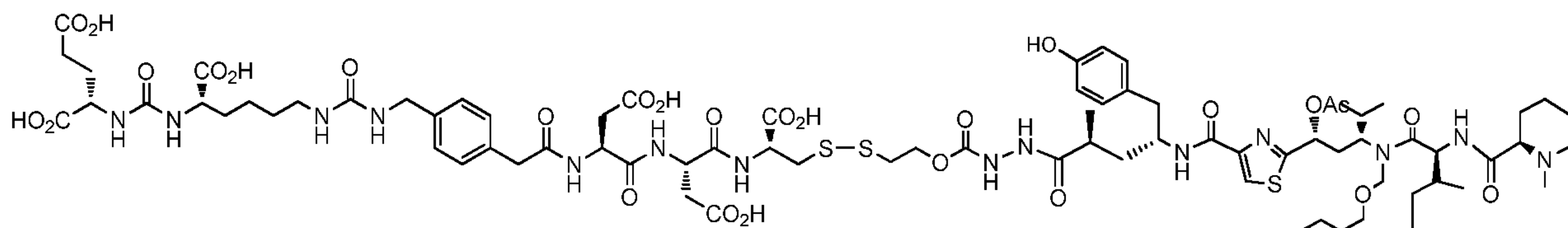
5 EC1677 (C 78 H 114 N 14 O 27 S 3 , Exact Mass: 1774.71, Molecular Weight: 1776.01)
