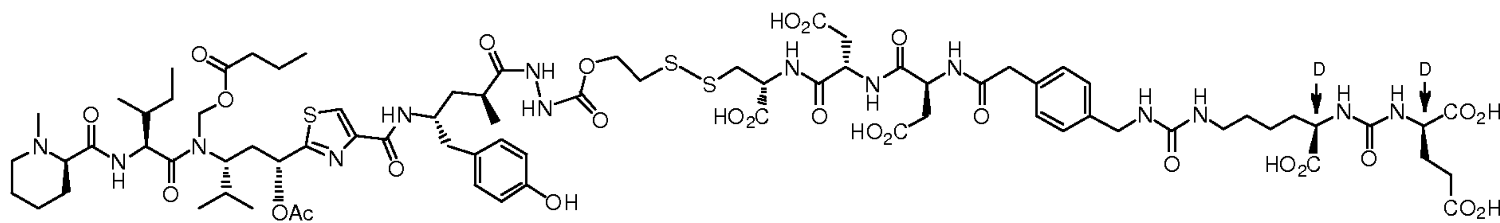
EC1268 (C 78 H 112 N 14 O 28 S 3 , Exact Mass: 1788.69, Mol. Wt.: 1790.00)
