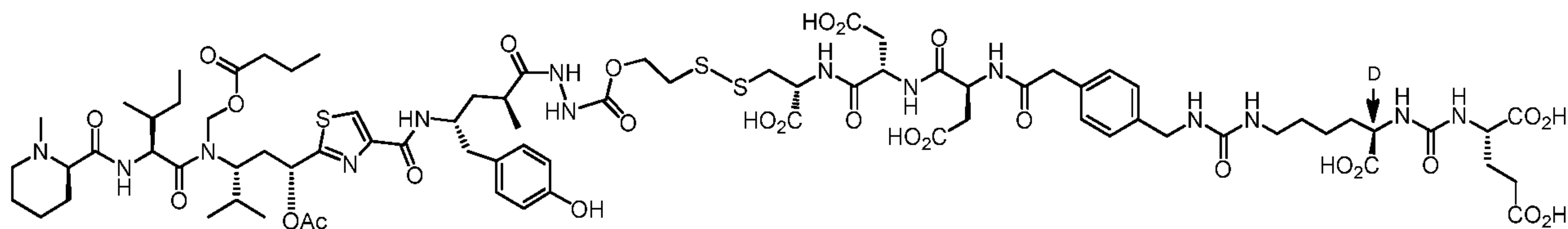
EC1269 (C 78 H 112 N 14 O 28 S 3 , Exact Mass: 1788.69, Mol. Wt.: 1790.00)
