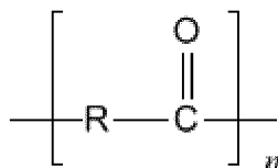
[Chemical Formula 2]
