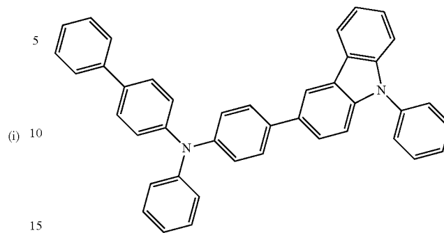
PCBA1BP
