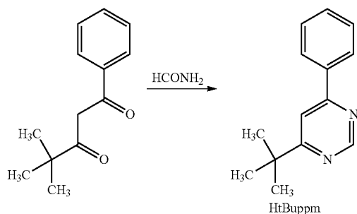
Step 2: Synthesis of Di- \mu -chloro-bis[bis(6-tert-butyl-4-phenylpyrimidinato)iridium(III)] (abbreviation: [\text{Ir}(\text{tBuppm})_2\text{Cl}]_2 )
