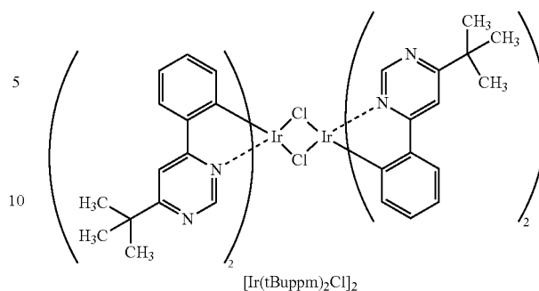
Step 3: Synthesis of (Acetylacetonato)bis(6-tert-butyl-4-phenylpyrimidinato)iridium(III) (abbreviation: [\text{Ir}(\text{tBuppm})_2(\text{acac})] )
