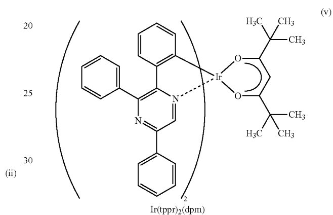
Ir(tppr) 2 (dpm)
