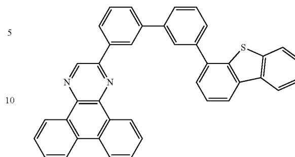
2mDBTBPDBq-II
