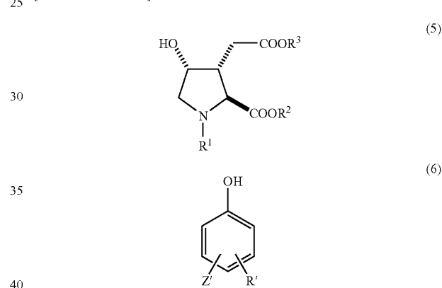
[Chemical Formula 6]
