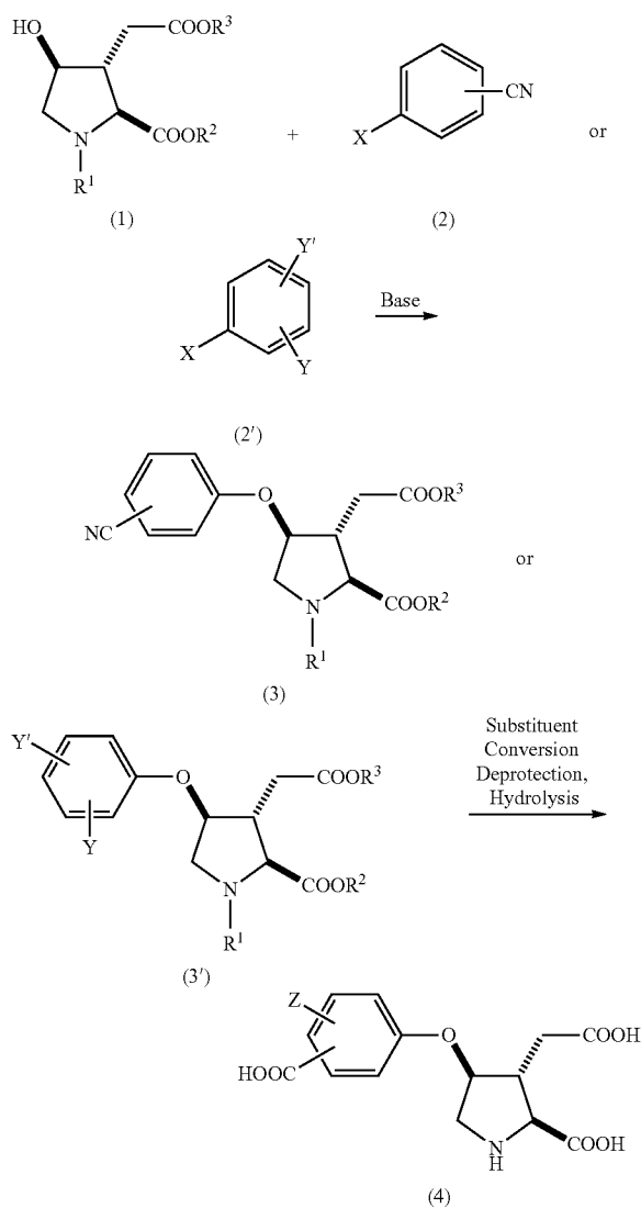
[Chemical Formula 5]
