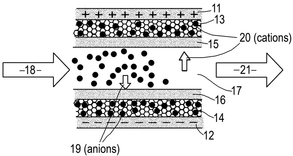
Fig.2 CDI Assembly
