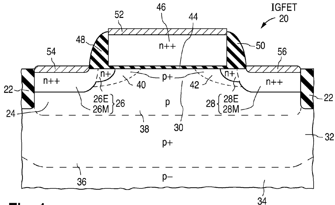
Fig. 1 PRIOR ART
