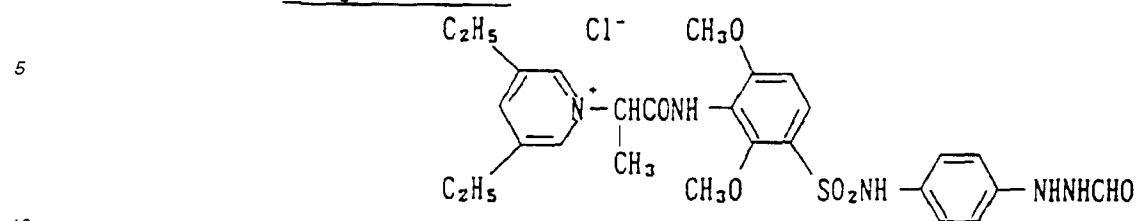
Compound 35:
