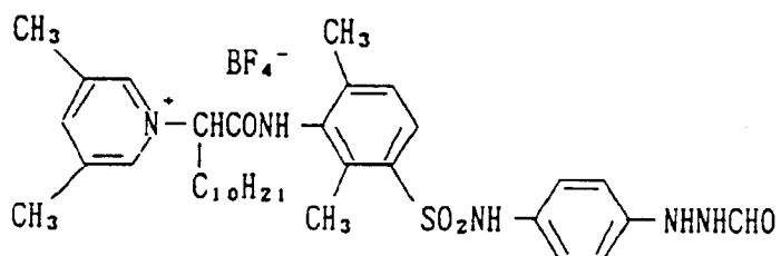
Compound 25:
