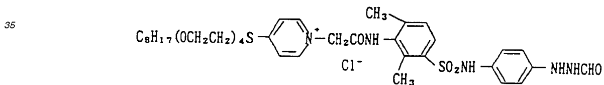
Compound 6:
