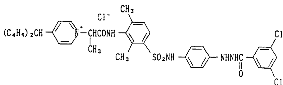
Compound 34:
