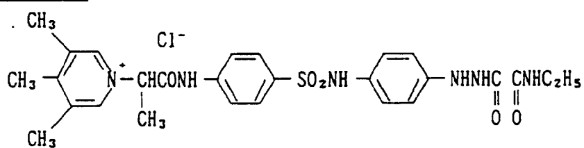
Compound 29:
