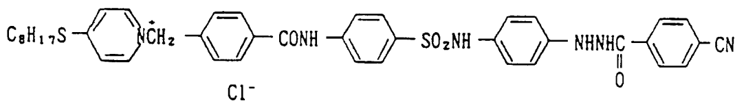
Compound 11:
