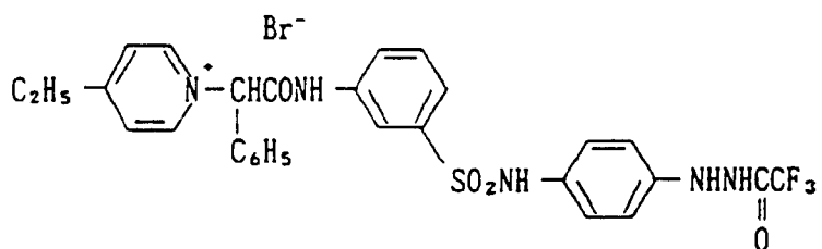
Compound 30:
