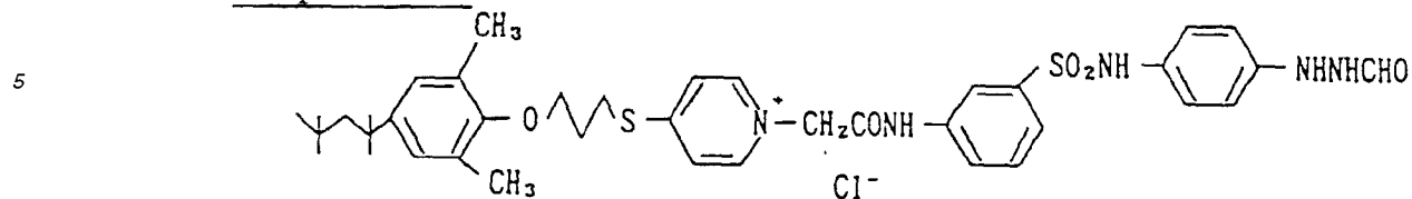
Compound 3:
