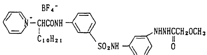
Compound 33:
