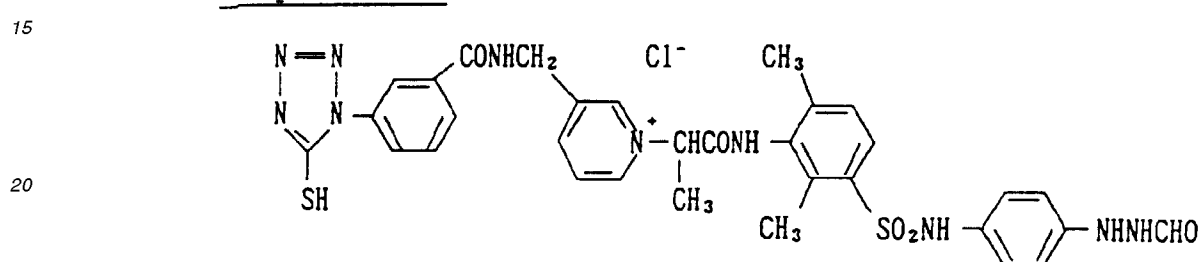
Compound 36:
