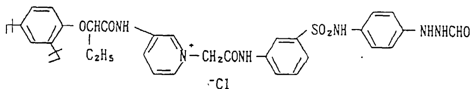
Compound 2:
