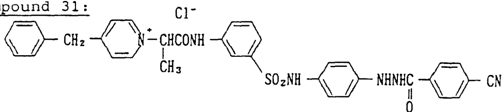
Compound 31:
