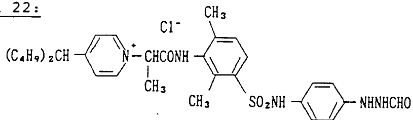
Compound 23:
