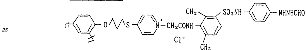
Compound 5:
