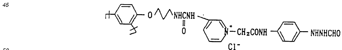
Compound 7:
