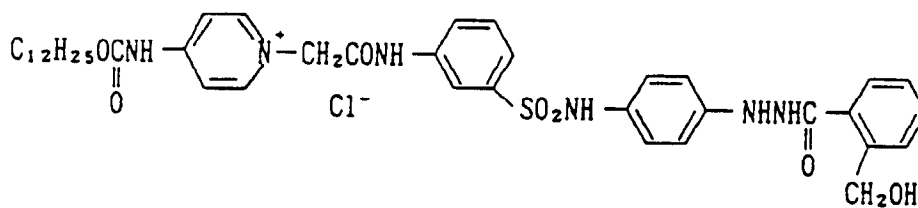
Compound 8:
