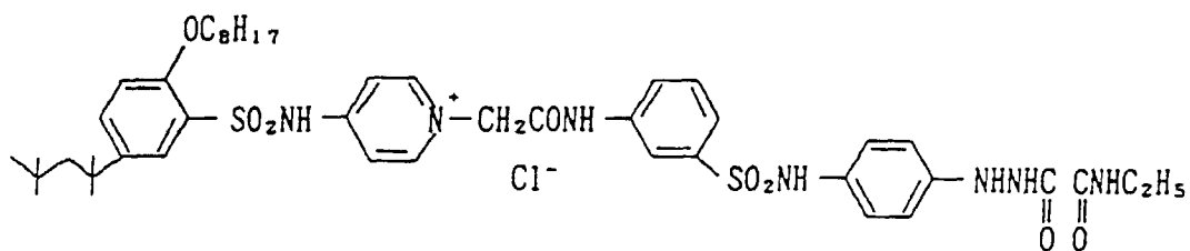
Compound 11:
