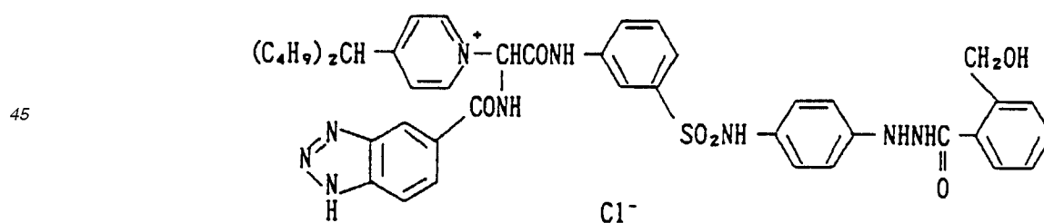
Compound 38:
