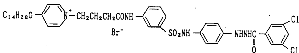
Compound 9:
