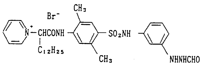
Compound 24:
