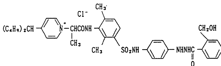
Compound 28:
