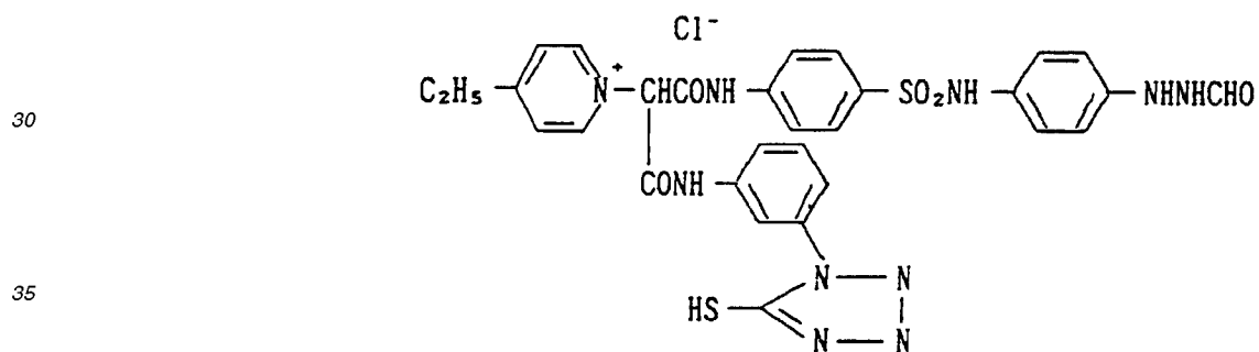
Compound 37:
