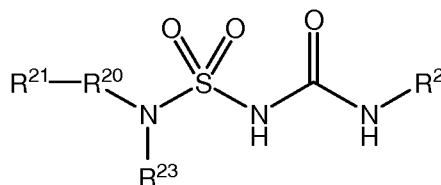
Formula (ID)
