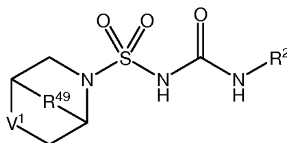
Formula (IB2)
