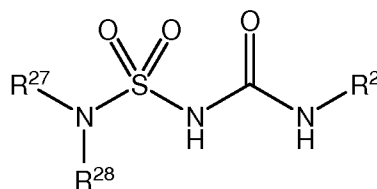
Formula (IF)
