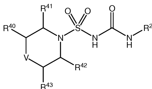
Formula (IB)
