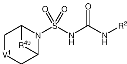
Formula (IB3)
