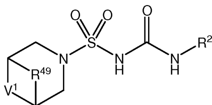
Formula (IB1)
