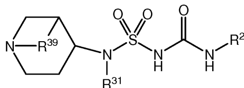
Formula (IE5)
