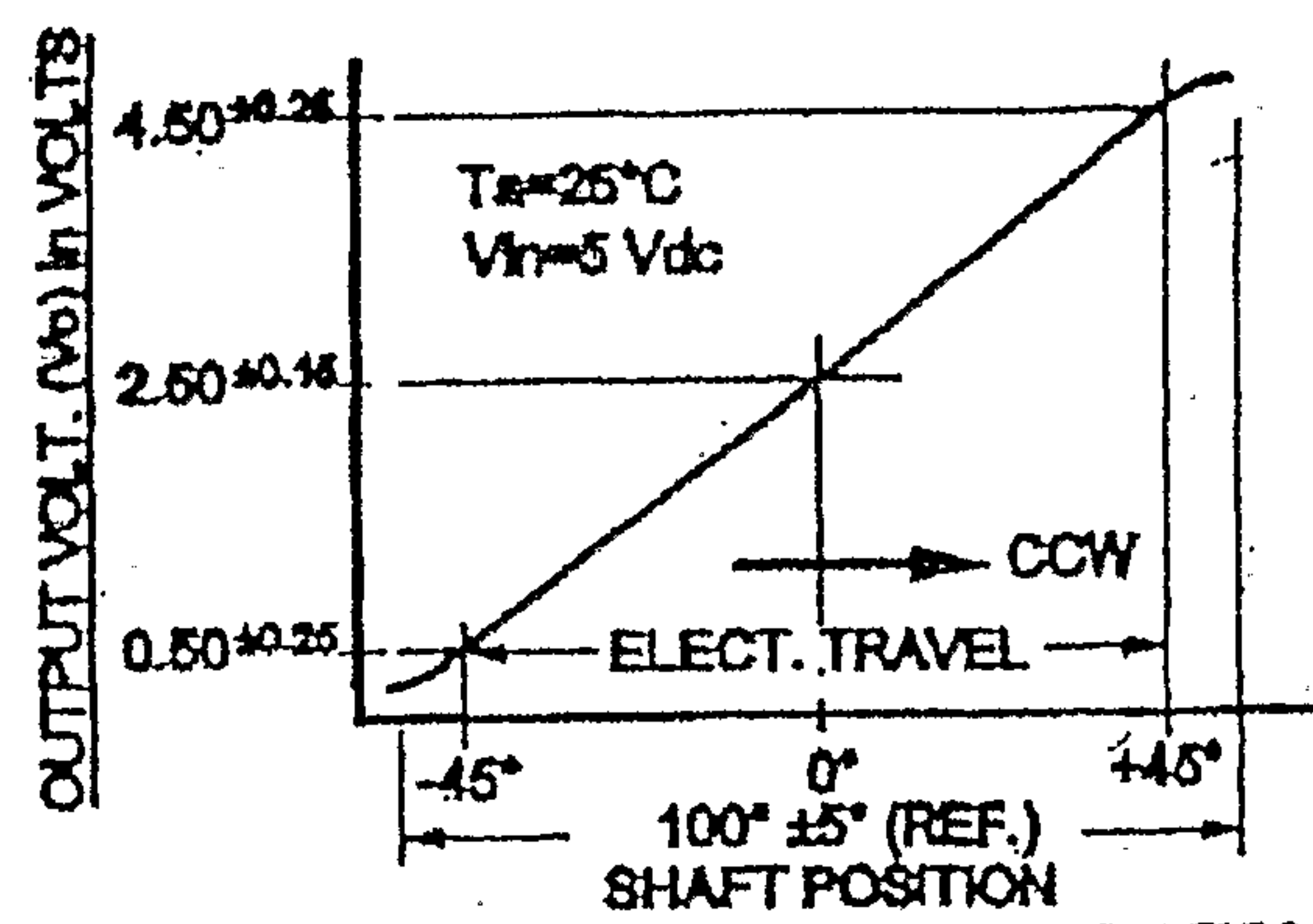
FIGURE 3 OUTPUT CHARACTERISTICS
