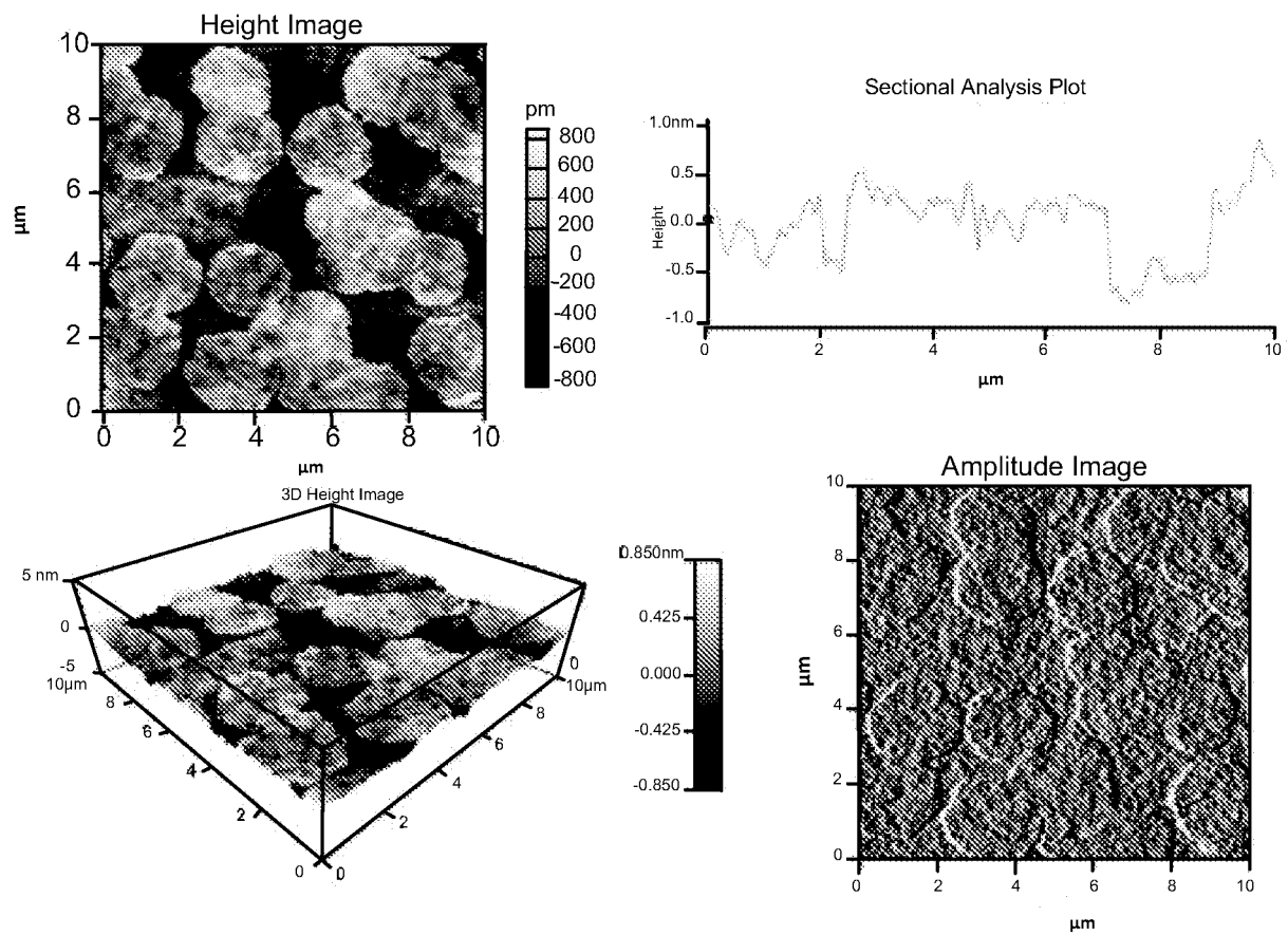
AFM Images of Glass Cover Slip
