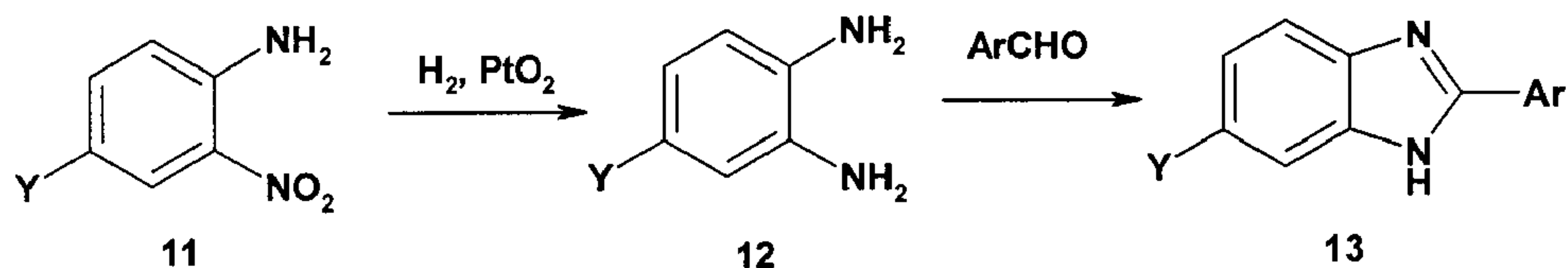
Scheme 3.
