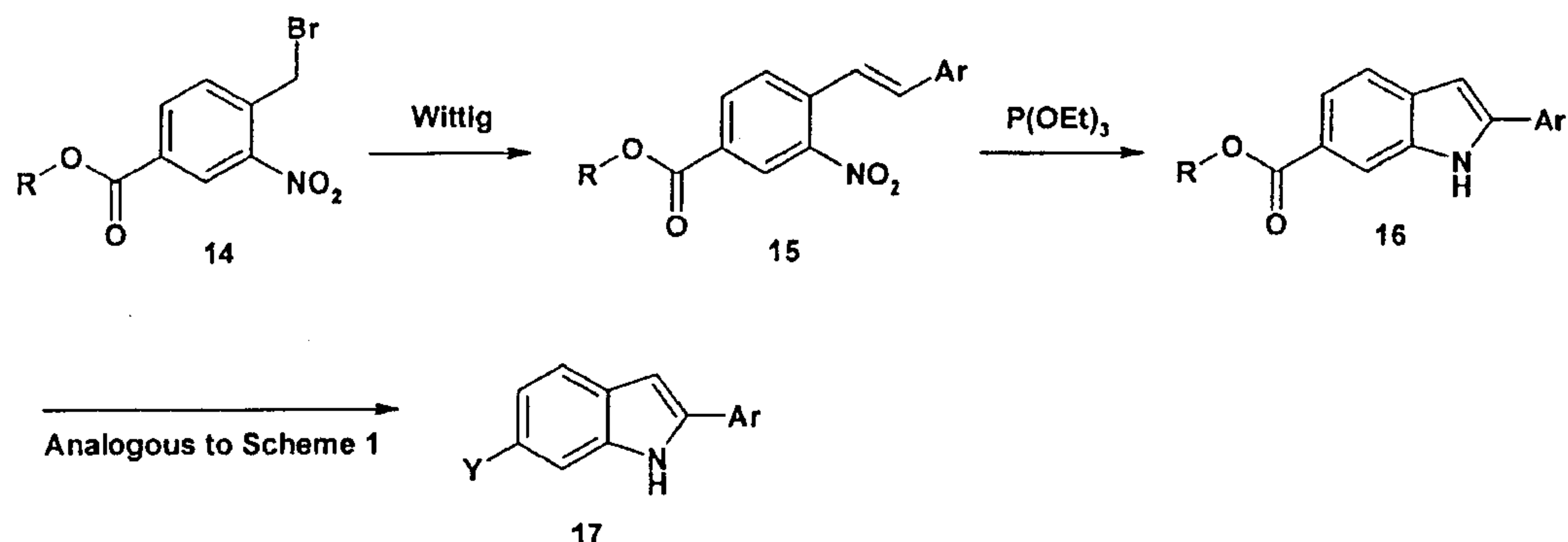
Scheme 4.
