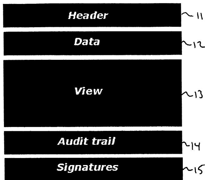
Figure 1: SMARTDoc Hierarchy
