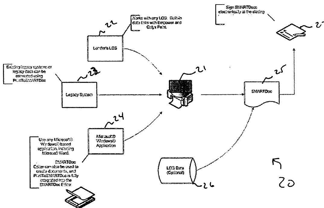
Figure 2: PrintToSMARTDoc Process
