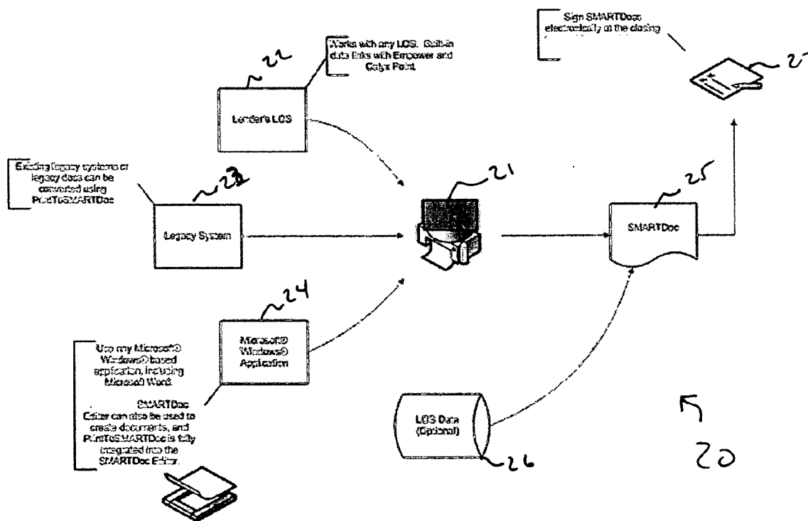
PrintToSMARTDoc Process
