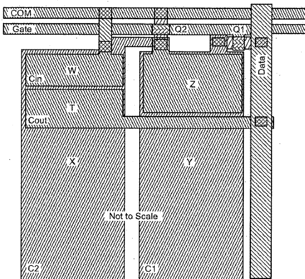
Subpixel Layout
