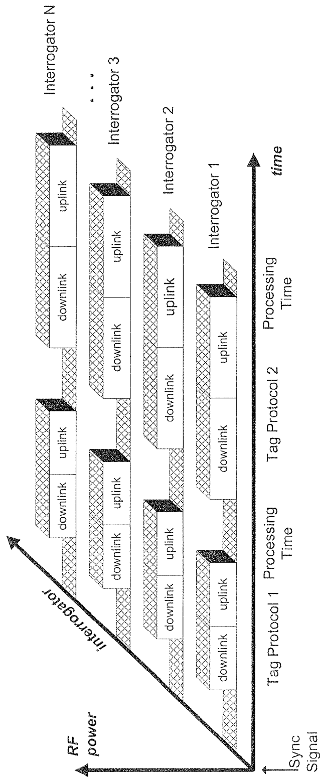
Figure 3(a) – Step Lock Timing Diagram
