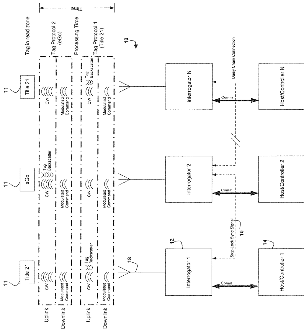
Figure 1 Step-Locked Interrogator Cluster (Internal Sync Signal)
