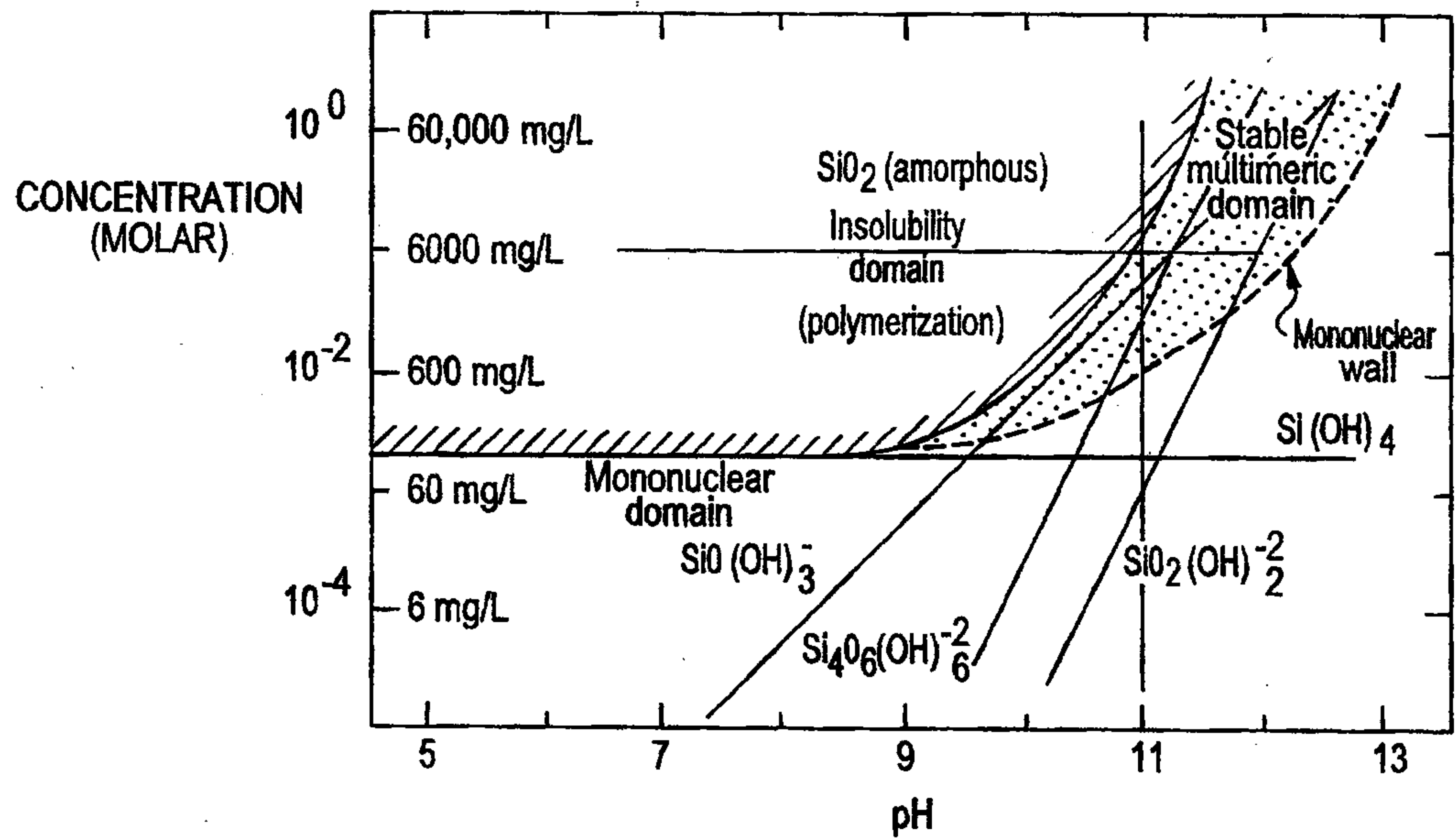
FIG. 11 SILICA SOLUBILITY CHARACTERISTICS
