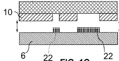
FIG. 1C (PRIOR ART)
