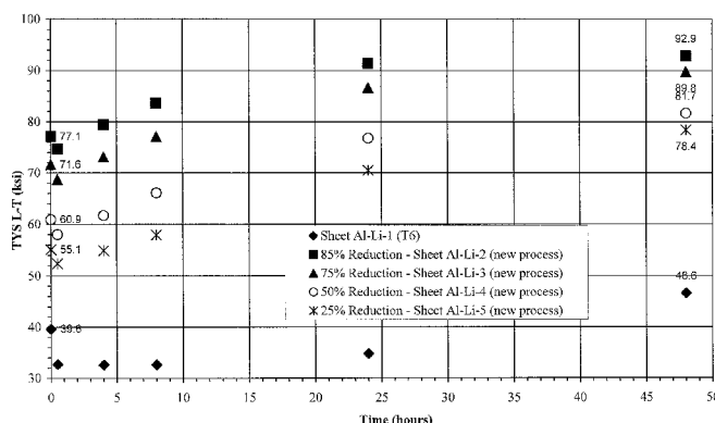
FIG. 15 - 2xxx Al-Li - TYS v. Time at 290F
