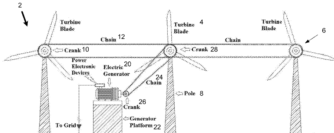
Figure: Wind Generator with Multiple Turbines (Rear View)
