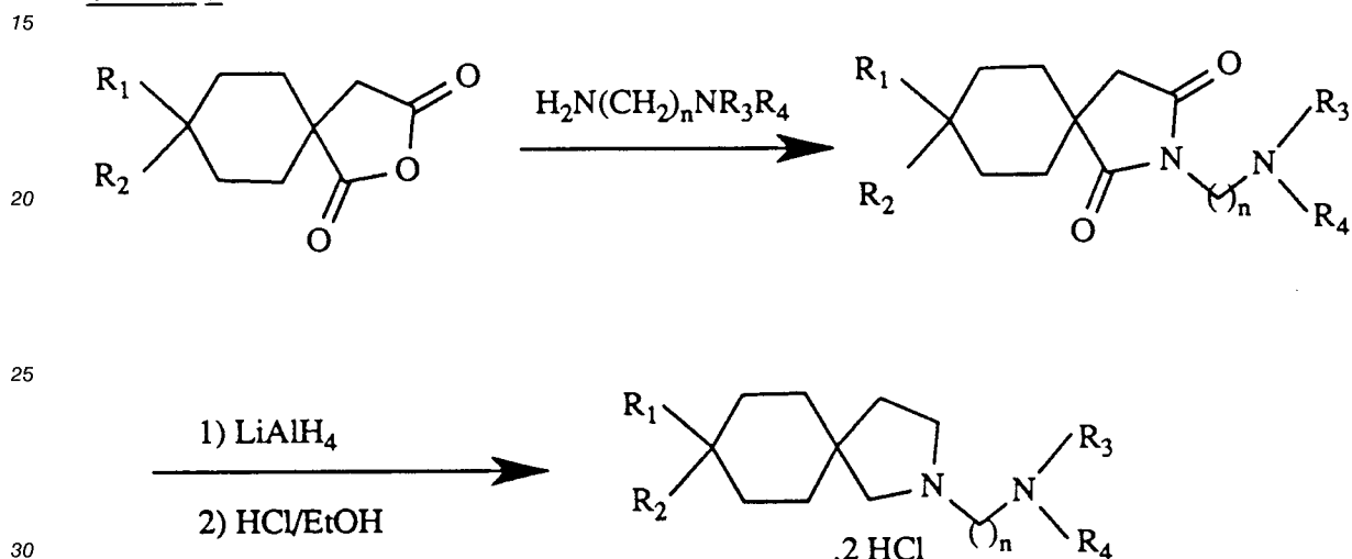
Scheme 5
