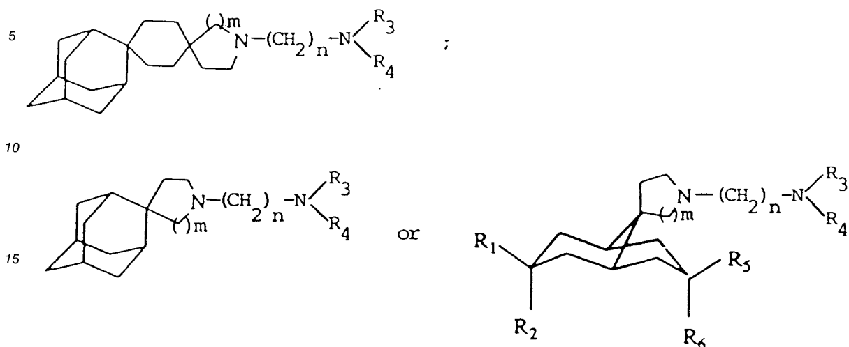
Formulae (II)
