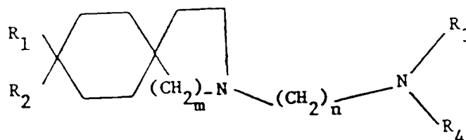
Formula (I)
