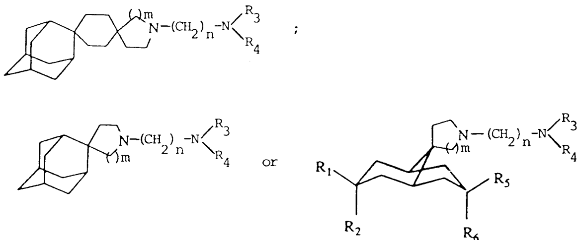
Formula (II)
