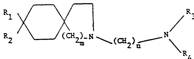
Formel (I)
