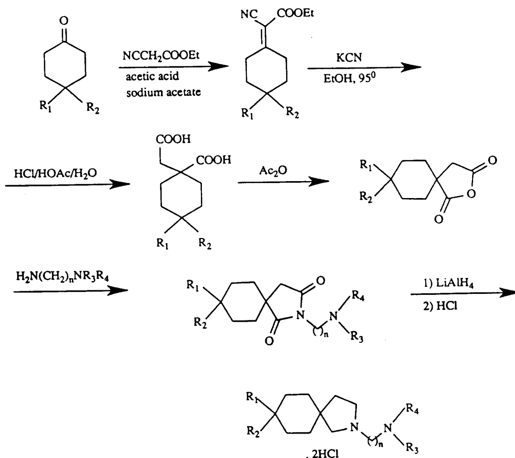
Scheme 3
