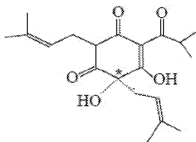
(+)-THCO
