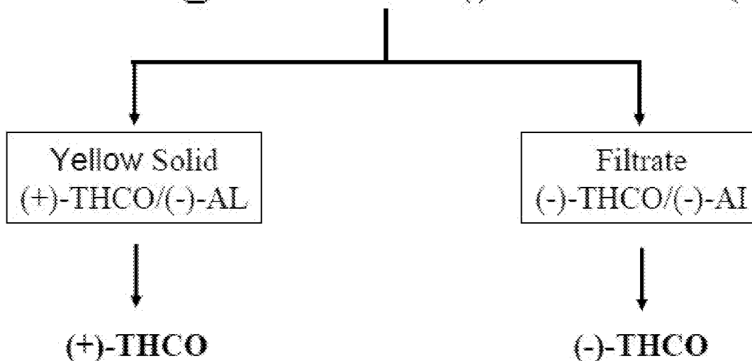
(+)-THCO
