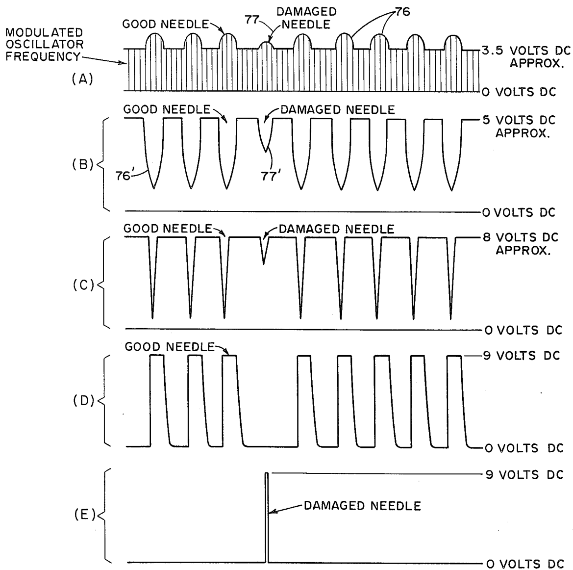
FIG. 5 WAVE FORMS
