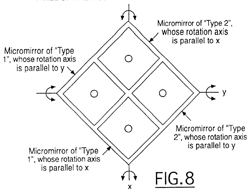
PIXEL OF THE MODIFIED MIRCOMIRROR DISPLAY
