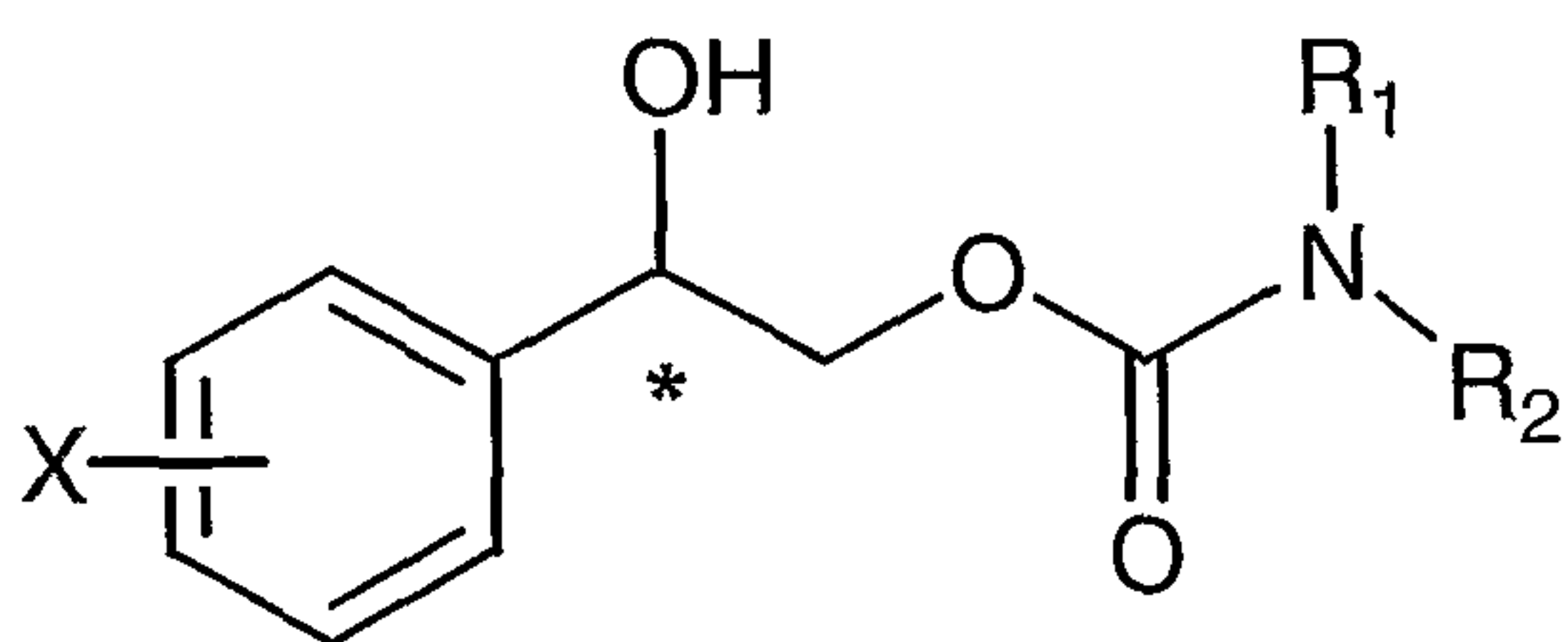
Formula (I)
