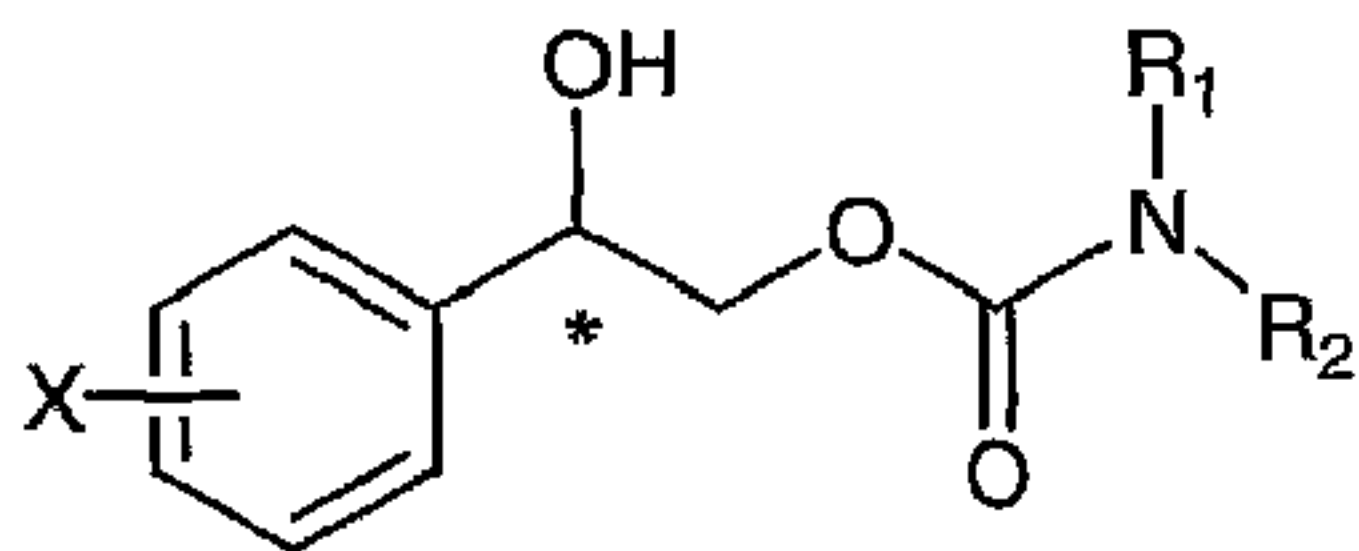
Formula (I)
