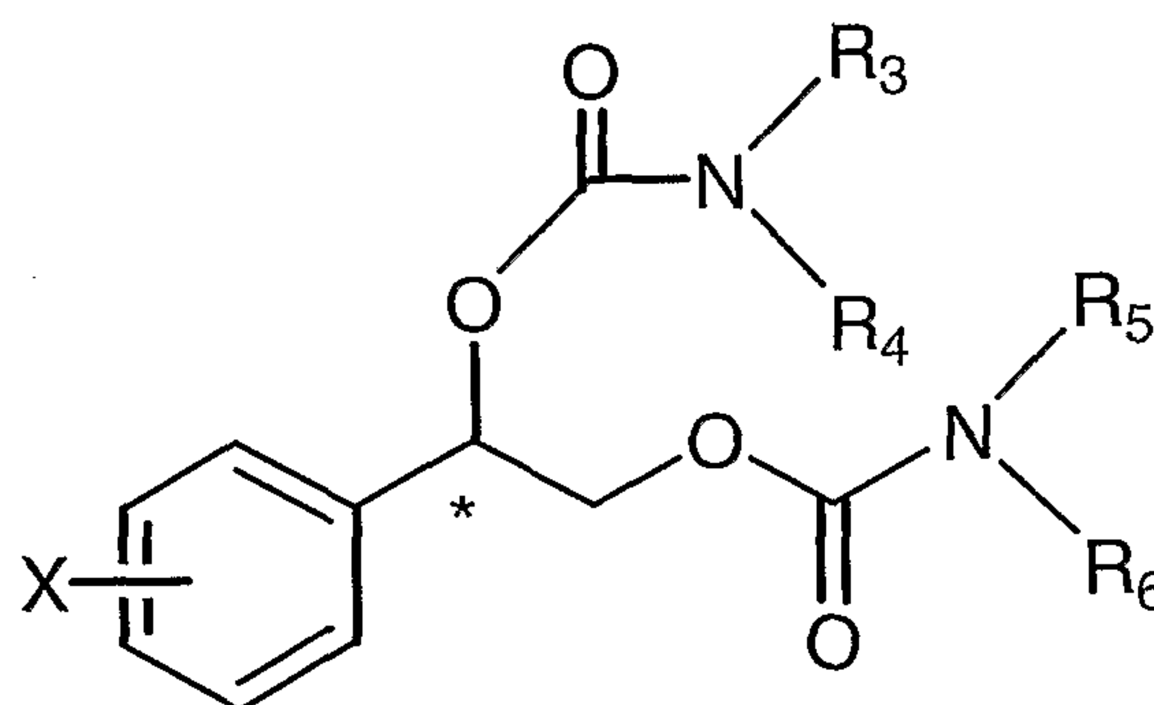
Formula (II)
