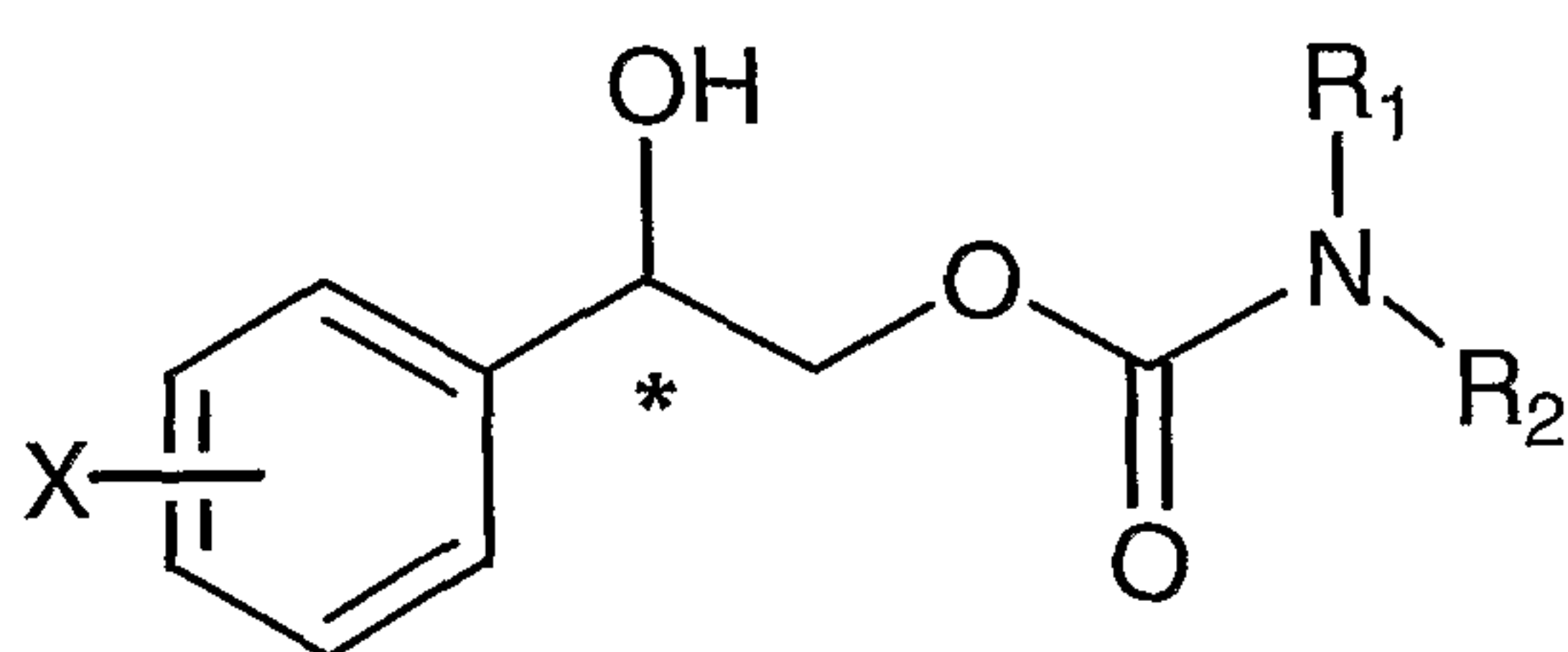
Formula (I)
