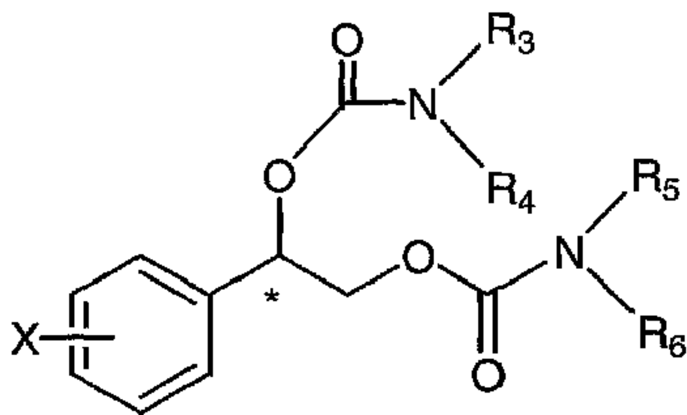
Formula (II)
