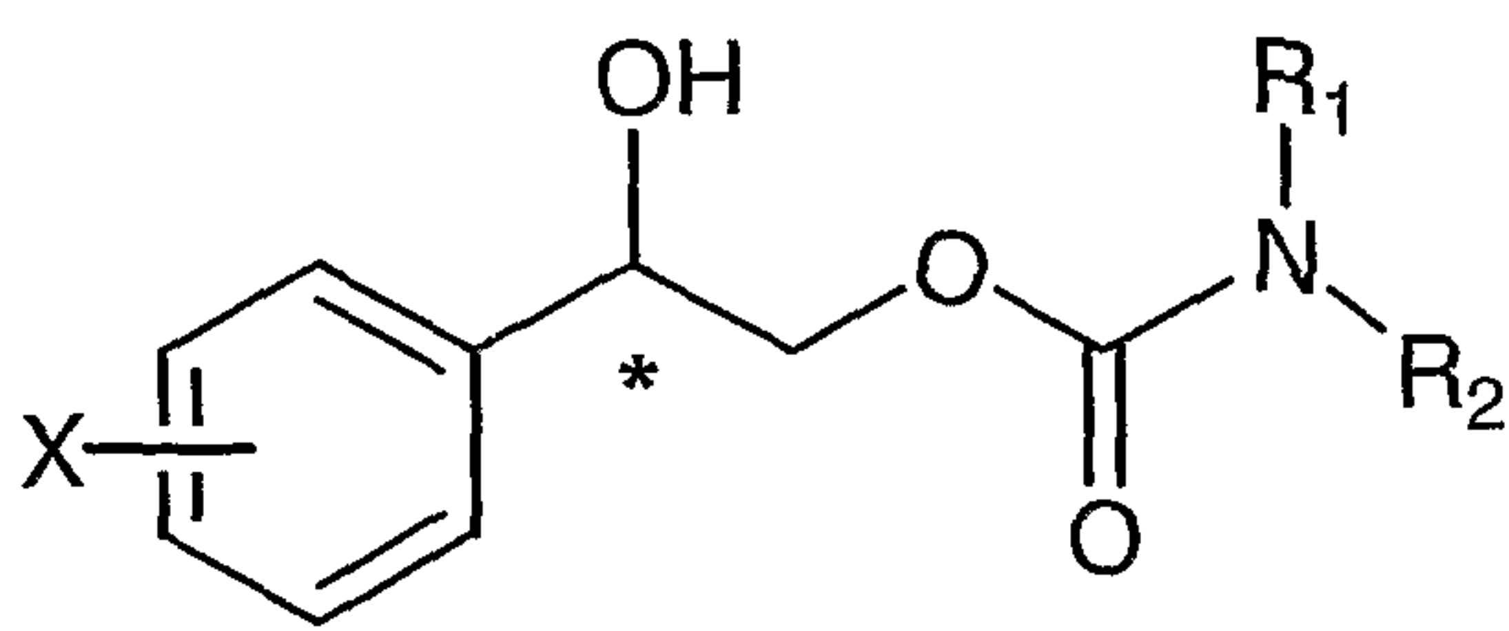
Formula (I)
