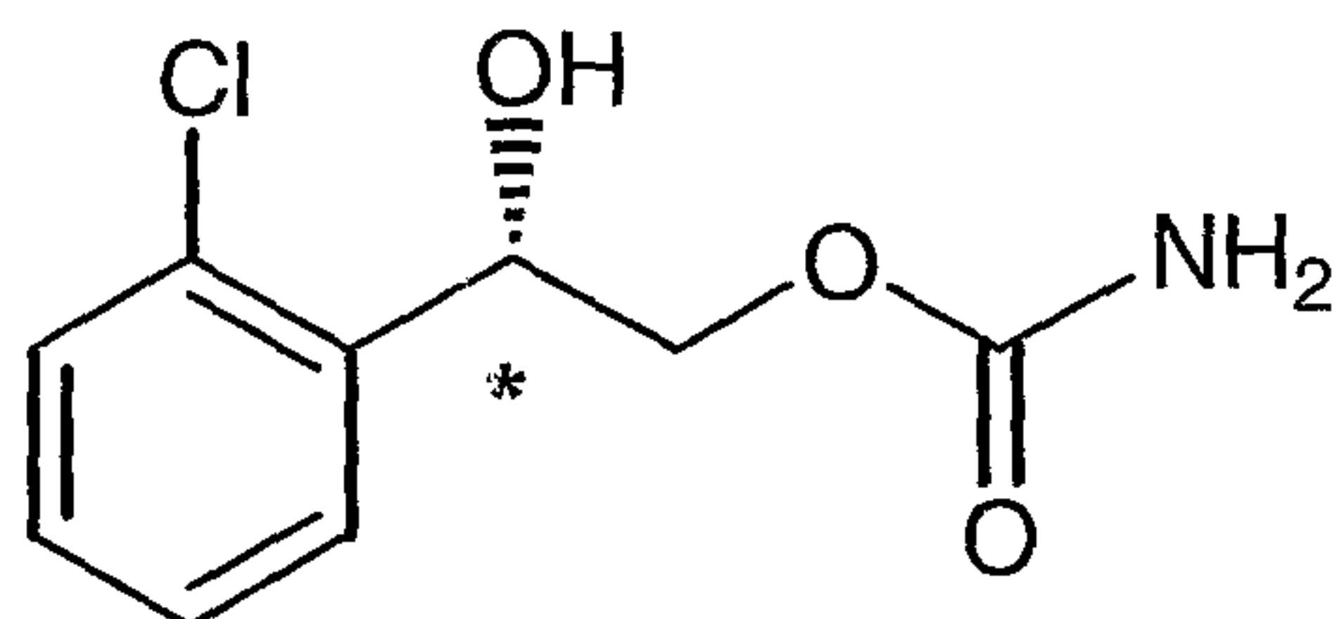
Formula (Ib)
