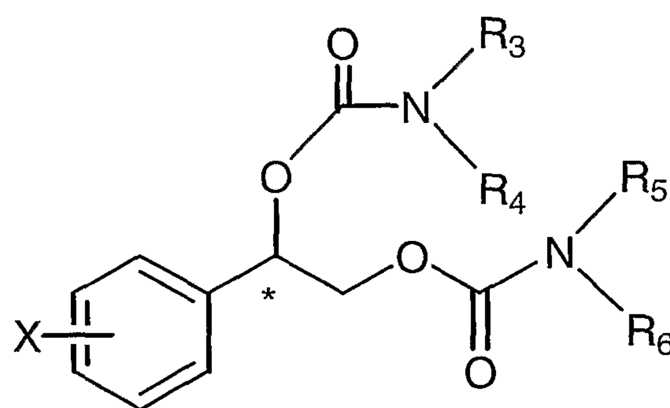
Formula (II)
