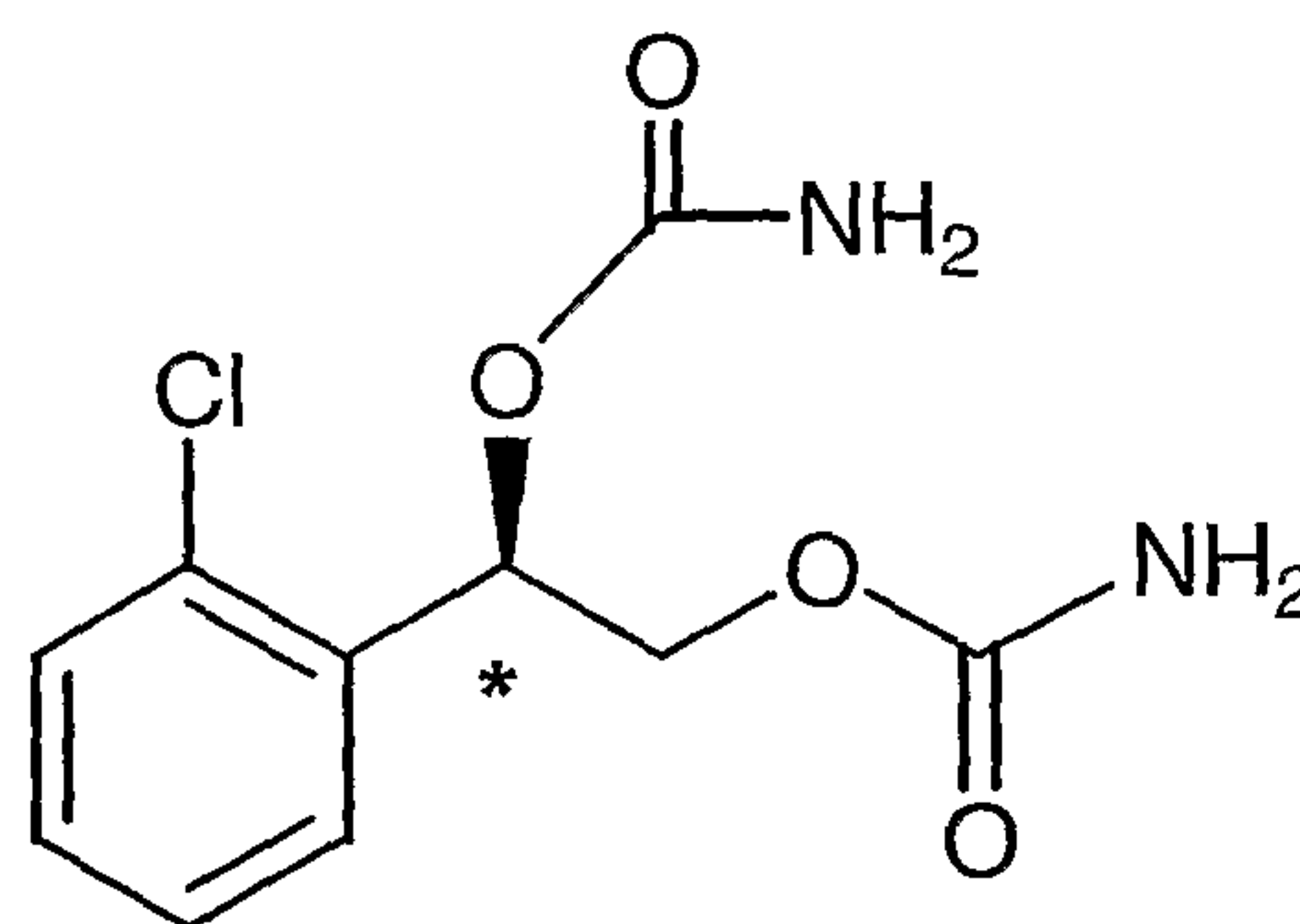
Formula (IIb)
