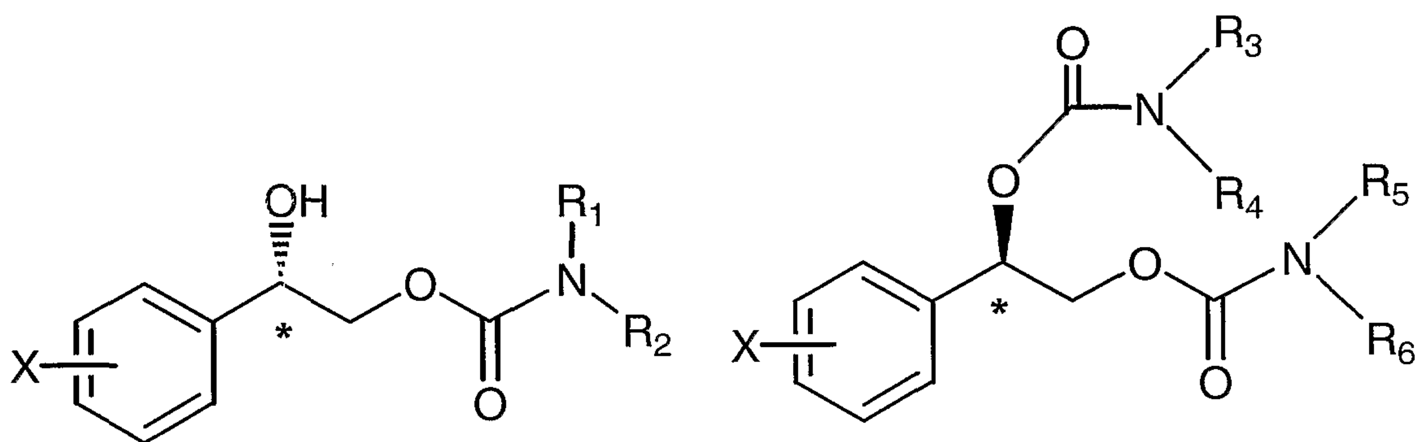
Formula (Ia)
