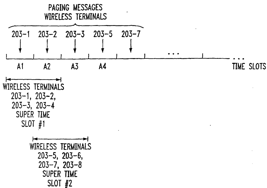
FIG. 7 PARTIALLY-OVERLAPPING SUPER TIME SLOTS
