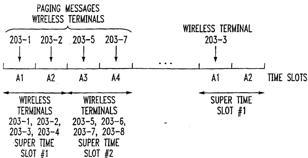
FIG. 6 NON-OVERLAPPING SUPER TIME SLOTS
