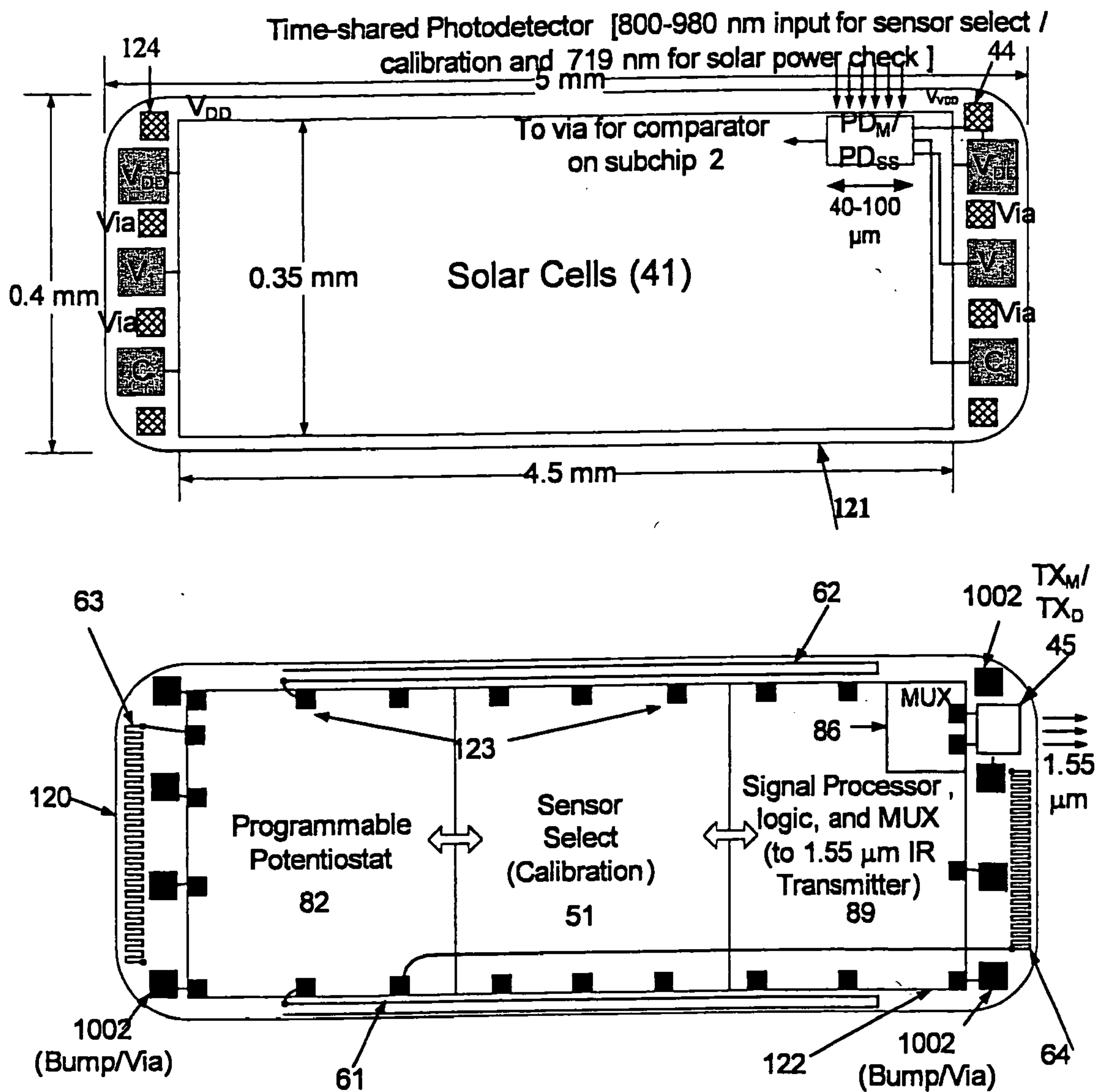
(i) Layout of two sub-chips.
