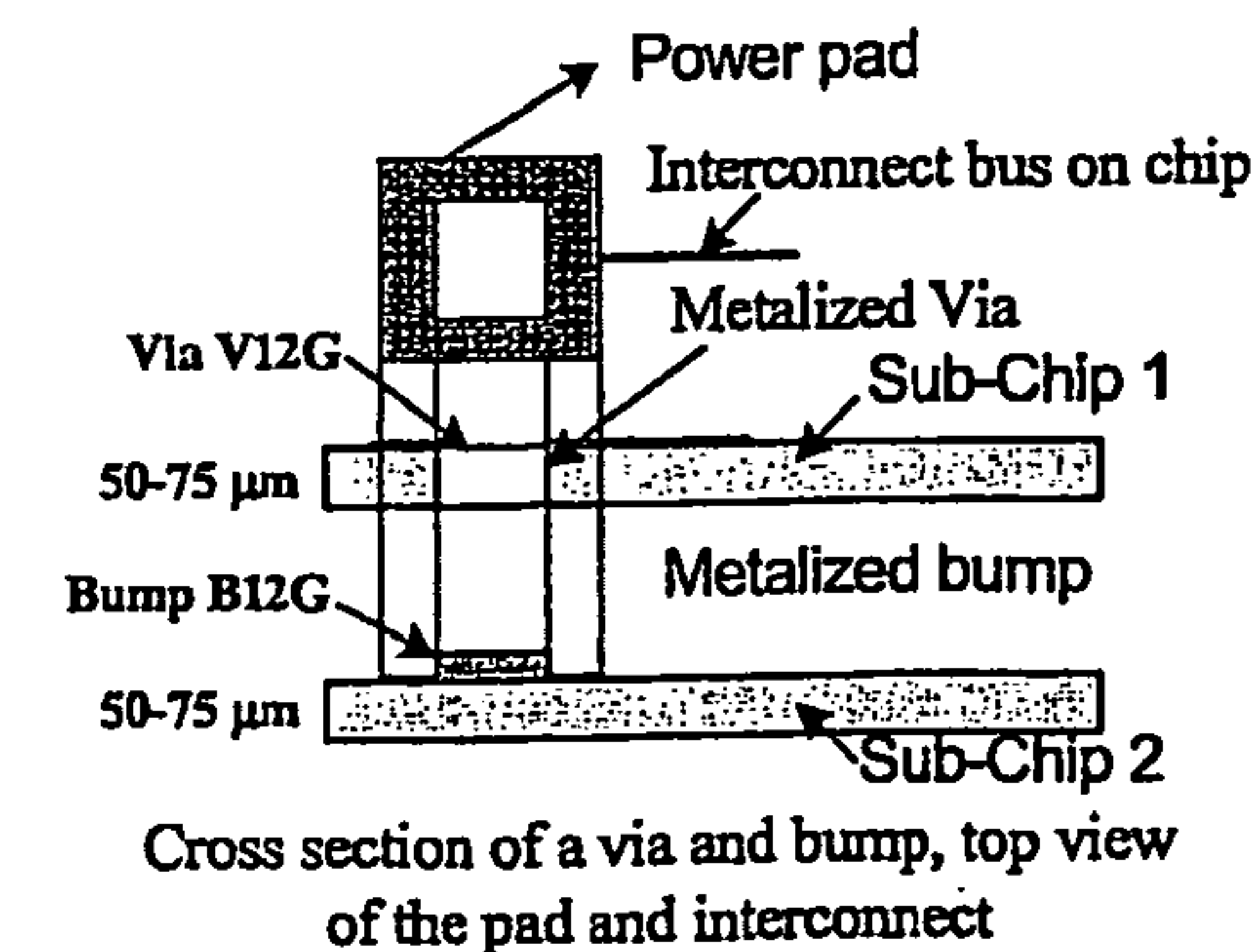
(i) Layout of two sub-chips.
