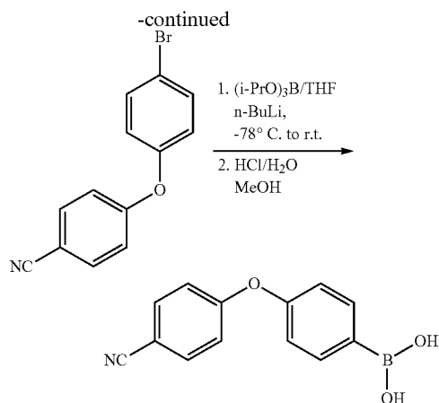
(a) (4-cyanophenyl)(4-bromophenyl)ether
