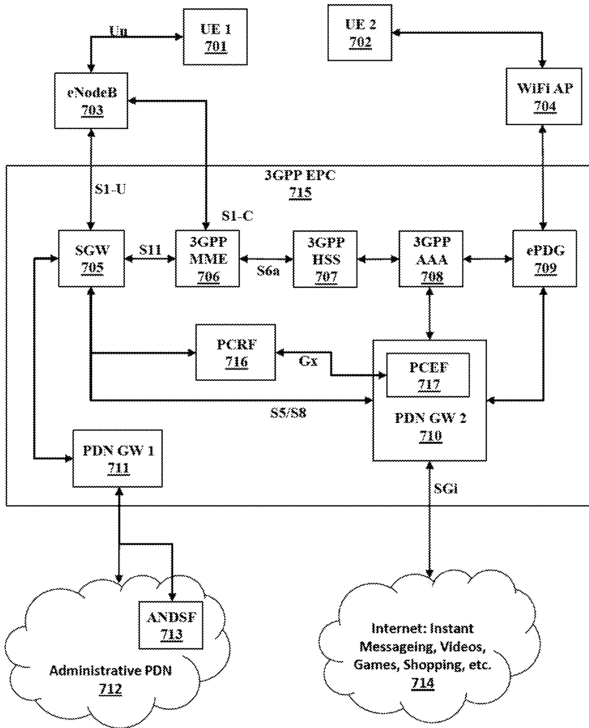
Fig. 7 (Prior Art)
