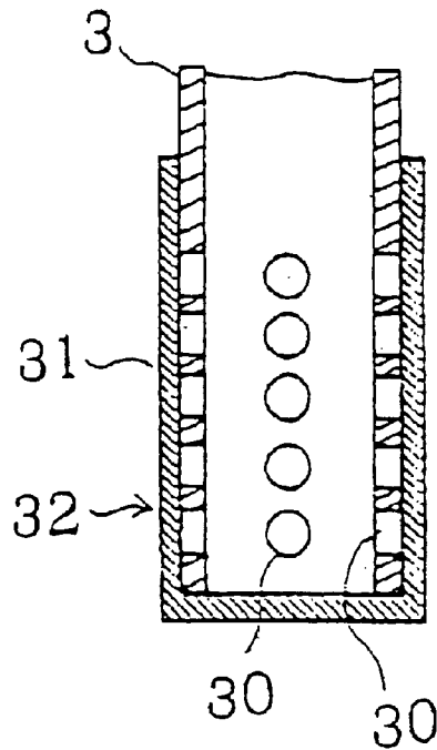
FIG. 3 PRIOR ART
