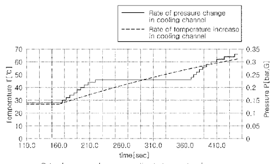
Rate of pressure change according to temperature increase in cooling channel when bubbles have been produced in coolant
