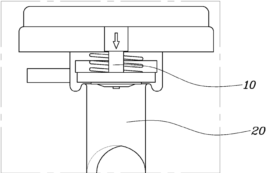
Valve closed
