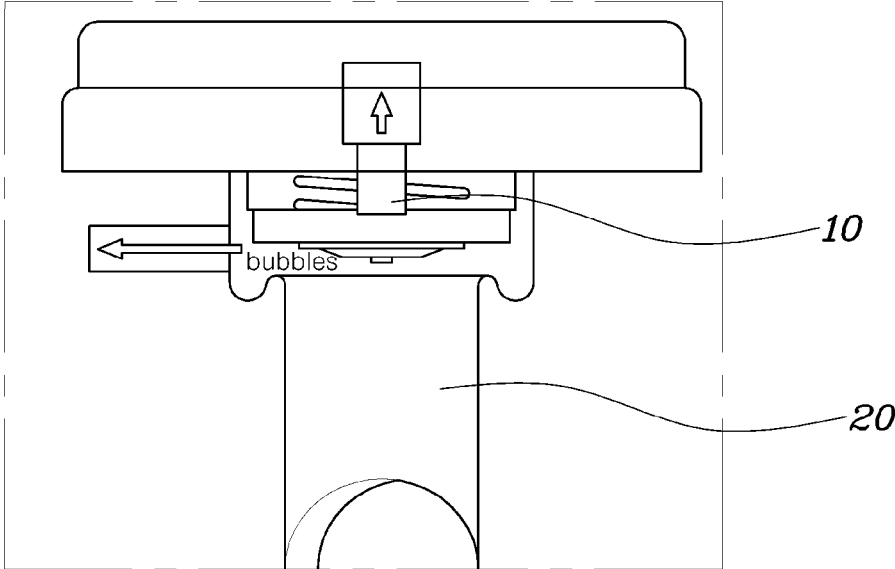
Valve open
