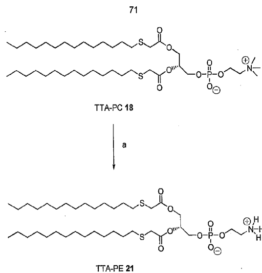
Scheme 5
