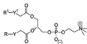
Phosphatidylcholine 1
