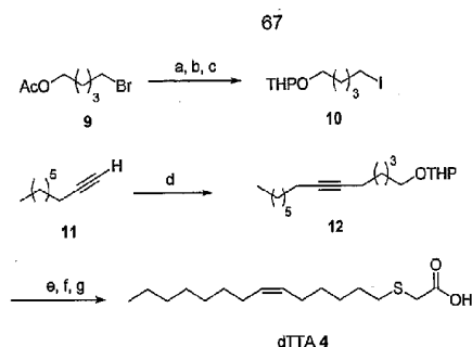
Scheme 2
