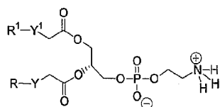
Phosphatidylethanolamine 2
