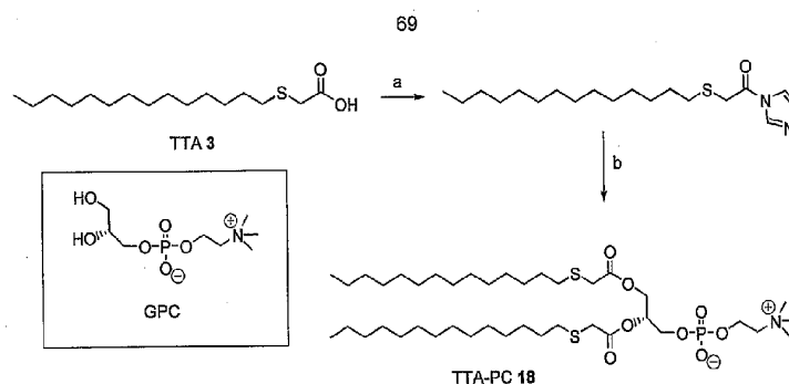
Scheme 4
