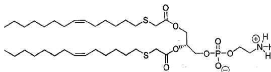
dTTA-PE 22
