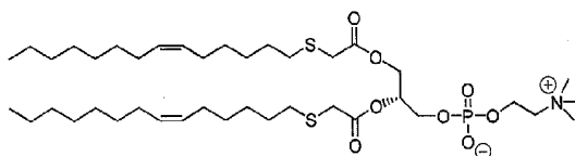
dTTA-PC 19
