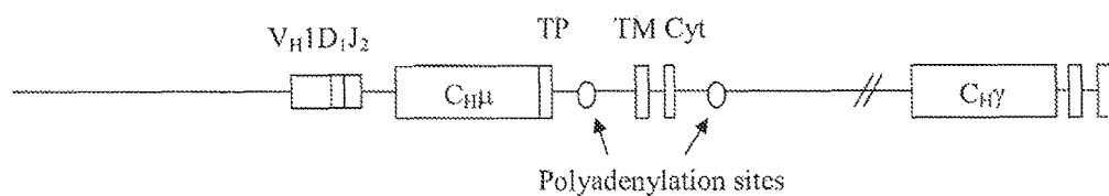
Figure 2C. Secreted and Membrane \mu -H Chains Encoded
