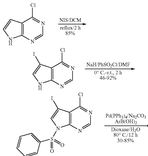
Scheme 1 General Synthesis of 5-Aryl pyrrolo[2,3-d]pyrimidine Compounds
