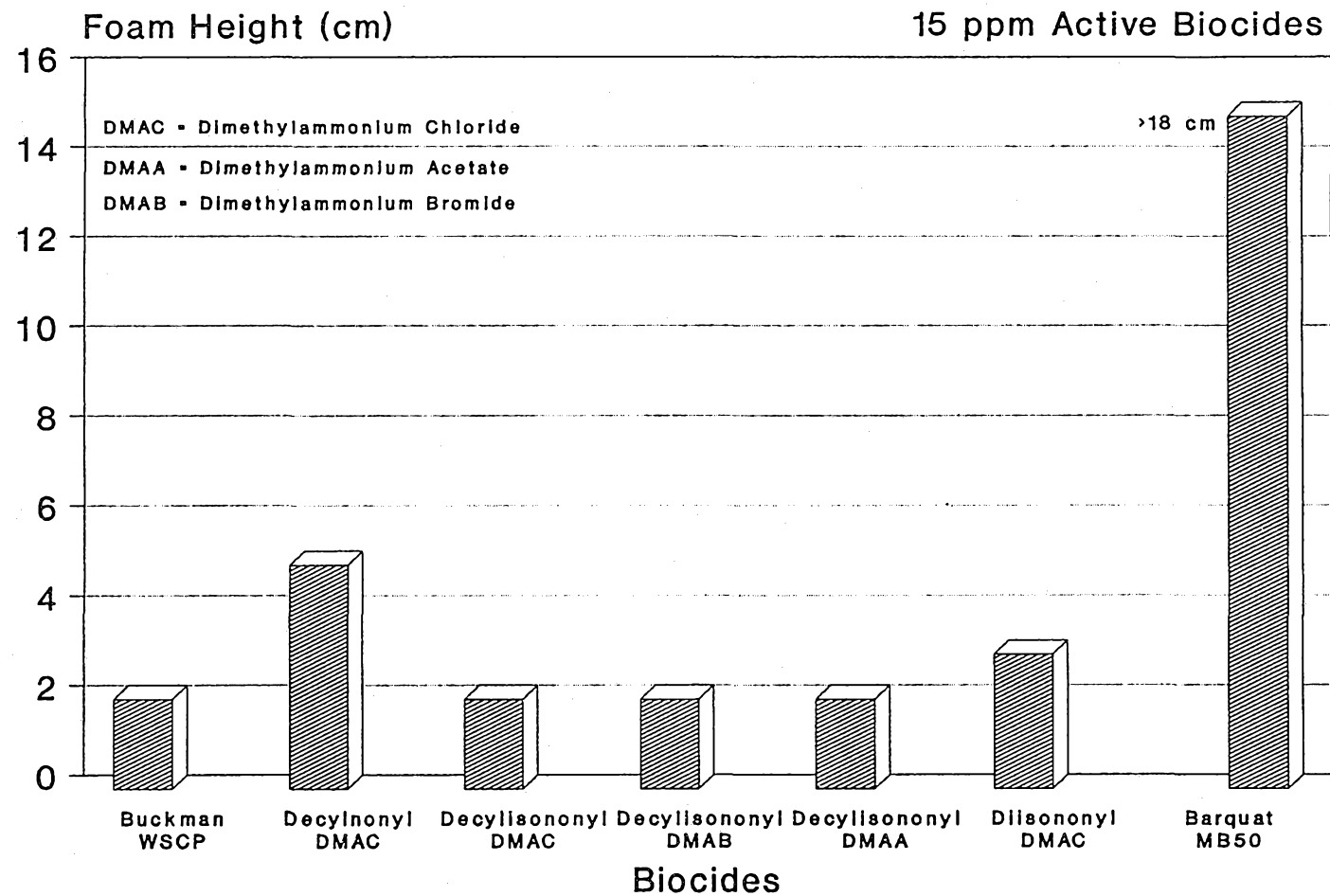
FIG. 6 - CIRCULATION FOAM TEST EQUIBRIUM FOAM HEIGHT
